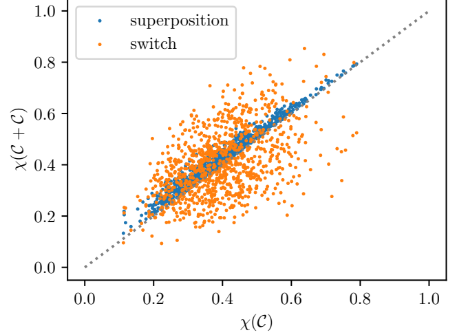
FIG. 5. Comparison of Holevo capacities of self-switch and self-superposition of 1000 random channels. Holevo capacity always increases in the latter case but no such regularity exists in the former. The + sign stands alternatively for \bowtie or \boxplus .
