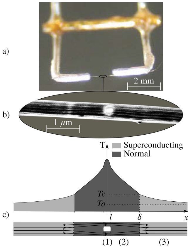
FIG. 1. Illustration and images of the hot-wire. (a) Picture of the wire stretched between the tips of the prongs. (b) Scanning electron microscopy picture of the NbTi wire with its reduced cross section drilled using a focused ion beam (central rectangular hole). (c) Typical temperature profile along the wire and schematic of the three regions of the wire in nominal operating conditions: (1) normal state with reduced cross section, (2) normal state, and (3) superconducting state.
