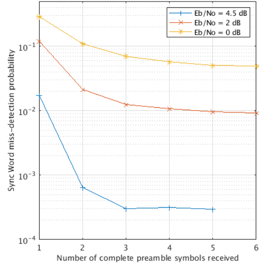
Fig. 7. Simulation (infinite precision) results showing the probability of sync word detection failure versus the number of complete un-modulated preamble symbols received by the receiver. Here sync word value is +8, SF = 7 , BW = 125 kHz, \alpha = 0.5 . STO_{int} and CFO are chosen randomly between [0, 1, \dots, 2^{SF} - 1] and \pm 34 ppm, respectively. SFO and STO_{frac} are set to zero.
