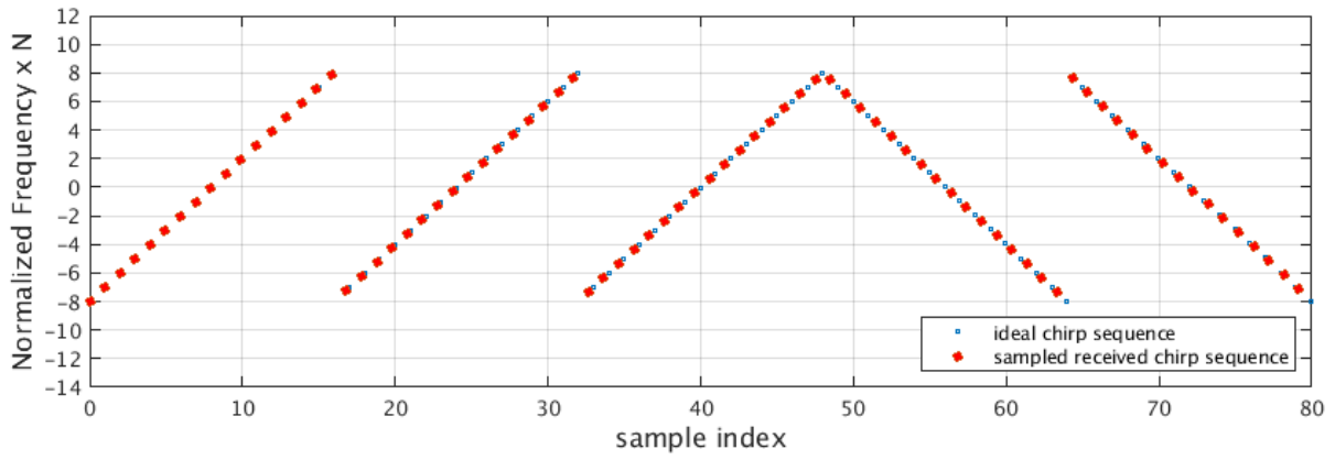
Fig. 4. Plot of N \times normalized frequency component of S_{N_0}(n) assuming N = 16 and N_0 = 0 and for a signal composed of three up-chirps and two down-chirps . Signal after sampling at a normalized rate of 1/N but with a small SFO (assuming STO and CFO = 0).
