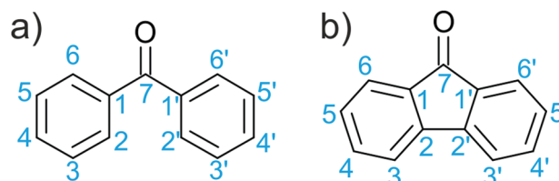
Fig. 1 (a) Benzophenone and (b) fluorenone. The numbers identify the C atoms.
