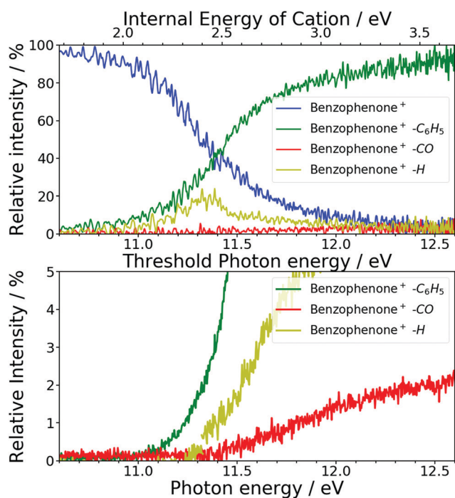
Fig. 7 Breakdown diagrams of the benzophenone cation fragmentation, built from the SPESs of Fig. 3 (top panel) and from the total ion yield of Fig. 4 (bottom panel). The full scale of this last graph is presented in the ESI.† These diagrams are relative and show the passage from parents to fragments. 43,44
