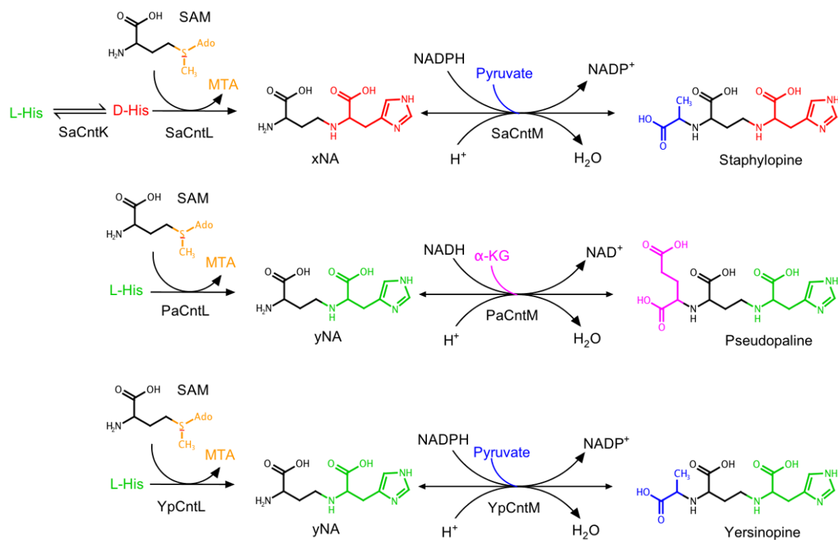
Figure 1: Differences in the staphylopine, pseudopaline, and yersinopine biosynthetic pathways. Adapted from [5,6,8].
