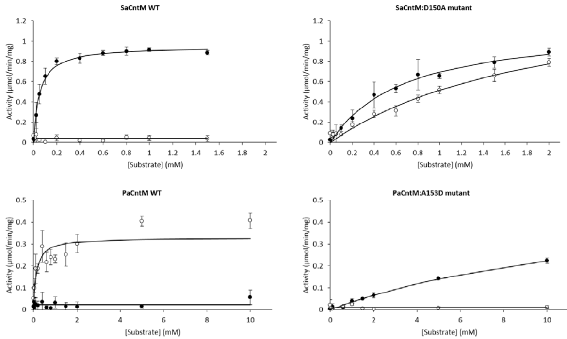
Figure 5: Activity profile of SaCntM (WT and D150A mutant) and PaCntM (WT and A153D mutant) using variable concentrations of pyruvate (black circle) and \alpha -ketoglutarate (white circle) with fixed concentrations of others substrates: 0.2 mM of NADPH and xNA when evaluating SaCntM, and 0.2 mM of NADH and yNA when evaluating PaCntM. The data points are means of three replicates with standard deviations. The fits are made using the Michaelis-Menten model.
