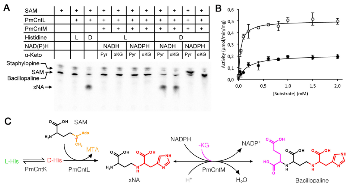
Figure 6: Activity of CntL and CntM from Paenibacillus mucilaginosus . (A) TLC separation of reaction products incubating carboxyl- ^{14}\text{C} -labeled with purified enzyme (PmCntL and PmCntM) and various substrates (L-His (L) or D-His (D), pyruvate (Pyr) or \alpha -ketoglutarate ( \alpha KG), NADH or NADPH). (B) Activity profile of PmCntM using variable concentrations of pyruvate (black circle) and \alpha -ketoglutarate (white circle) with fixed concentrations of others substrates: 0.2 mM of NADPH and 0.2 mM of xNA. The data points are means of three replicates with standard deviations. The fits are made using the Michaelis-Menten model. (C) Biosynthetic pathway for the assembly of bacillopaline from D-His, SAM and \alpha -ketoglutarate.
