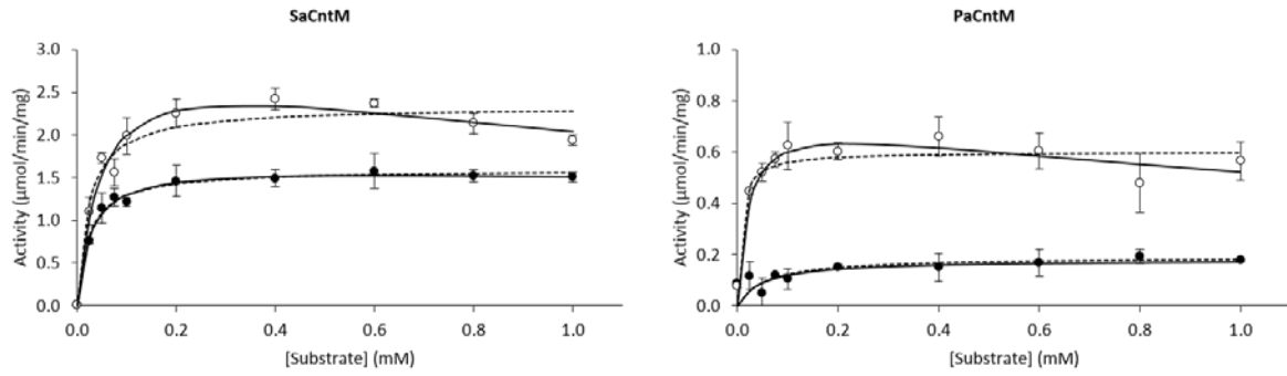
Figure 4: Activity profile of SaCntM and PaCntM using variable concentrations of xNA (black circle) and yNA (white circle) with fixed concentrations of other substrates: 0.2 mM of NADPH and 1 mM of pyruvate when evaluating SaCntM, or 0.2 mM of NADH and 1 mM of \alpha -ketoglutarate when evaluating PaCntM. The data points are means of three replicates with standard deviations. The fits are made using the Michaelis-Menten model considering (continuous line) or not (dashed line) a substrate inhibition.
