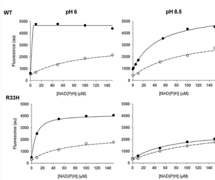
Figure 3: Titration of NADPH (black circles) and NADH (white circles) binding to SaCntM (5 \mu M) at pH = 6.0 or pH = 8.5 followed by fluorescence energy transfer between tryptophan excitation (280 nm) and NAD(P)H emission (450 nm).
