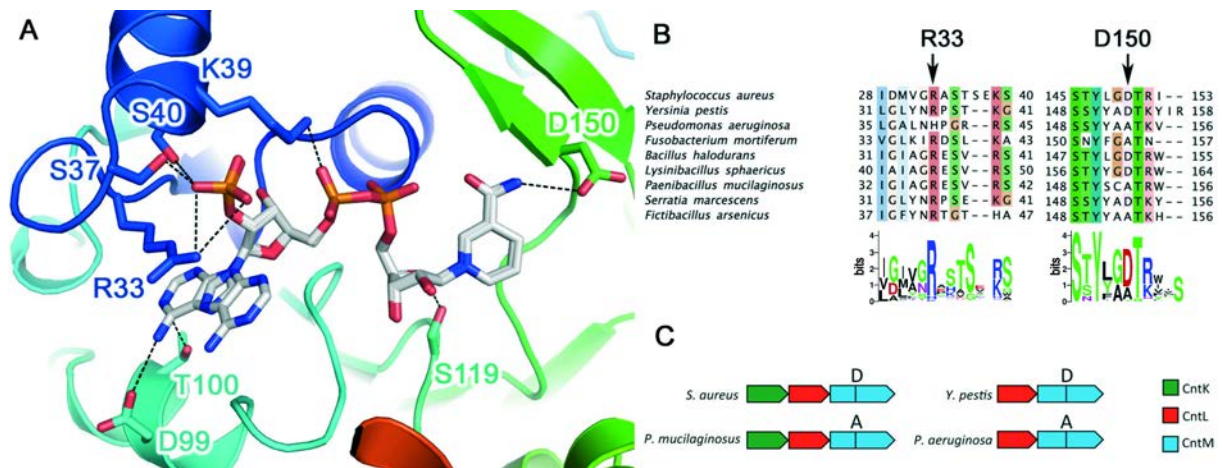
Figure 2: CntM structure, sequence conservation around NADPH and operon diversity highlight protein selectivity. (A) Details of the NADPH binding site on SaCntM with side chains of residues located up to 4Å around the NADPH represented in stick. The protein is colored from N-terminus (blue) to C-terminus (red). The pdb code used for this figure corresponds to 6H3D and shows two alternative positions for the adenine moiety of NADPH. Dashed lines indicate hydrogen bonds and salt bridges. The nicotinamide moiety is where the reductive condensation of xNA with pyruvate occurs and is involved in a putative hydrogen bond with D150 side chain. (B) Sequence alignment of nine CntM protein sequences from bacteria. Threshold for the Clustal coloring scheme correspond to 30 % sequence conservation as defined in Jalview. Arrows point to residues involved in NADPH/NADH selectivity and pyruvate/ \alpha -ketoglutarate selectivity. A weblogo representation of the entire unitprot family available from Pfam (318 entries) is drawn below the alignment, showing the conservation of position equivalent to R33 (R: 90%, H: 6% and K: 4%) and D150 (D: 72%, A: 25% and T: 3%) (C) Genomic organization of the biosynthetic genes of four different cnt operons in bacteria.
