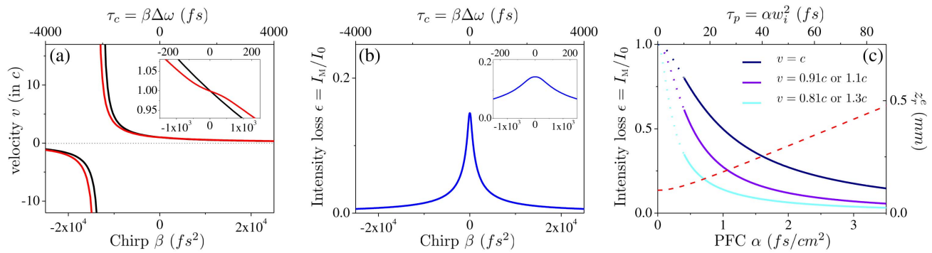
Fig. 4. Quantitative properties of CPLC beams, for \alpha = 3 \text{ fs}/\text{cm}^2 , \lambda_0 = 800 \text{ nm} , \tau_F = 25 \text{ fs} , w_i = 5 \text{ cm} , and f = 1 \text{ m} as in Fig. 3. (a) Propagation velocity v of the intensity peak of a CPLC beam around focus, as a function of chirp \beta . The black line corresponds to the prediction of Eq. (3), while the red one shows the velocity deduced from numerical simulations. (b) Corresponding peak intensity reduction factor \epsilon = I_M/I_0 as a function of \beta . In both panels, the insets show zooms on these curves for small values of \beta . (c) Peak intensity reduction factor \epsilon (full lines) as a function of \alpha , for fixed propagation velocities v = c , v = 1.1c or 0.91c , and v = 1.3c or 0.81c , corresponding to \beta/\alpha = 0 , \pm 7.71 \times 10^2 \text{ fs} \cdot \text{cm}^2 and \pm 1.95 \times 10^3 \text{ fs} \cdot \text{cm}^2 . The dotted parts of the curves correspond to a range where the calculation no longer makes sense, because PFC/LC becomes too weak. The red dashed line shows the evolution of the extended Rayleigh length z_r^e with \alpha , obtained from numerical simulations.
