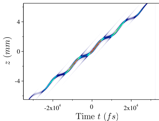
Fig. 5. Pulse with an oscillating propagation velocity produced using CPLC with a high-order spectral phase. Simulated on-axis spatio-temporal intensity profile I(z, t) , along the extended Rayleigh length, of a CPLC beam with an oscillating spectral phase, leading to a velocity v oscillating between c and 0.3c . Compared to Fig. 3, the PFC/LC parameter has also been increased to \alpha = 30 \text{ fs}/\text{cm}^2 ( \tau_P = 750 \text{ fs} ), while all other beam parameters are identical.
