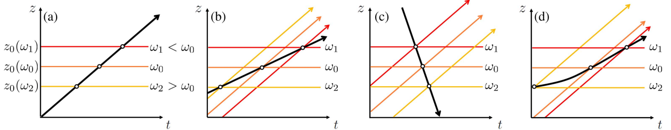
Fig. 2. How CPLC enable adjustable light pulse velocities. Because of PFC/LC, different frequencies of the pulse (here \omega_1 < \omega_0 < \omega_2 ) are focused at different longitudinal positions z_0(\omega) , indicated by the horizontal color lines. In (a), no chirp is applied, and the pulse intensity peak (black line with arrow) propagates at c . In (b), the frequencies that have their best focus at large z are retarded in time, leading to an effective velocity smaller than c . In (c), these same frequencies are now advanced in time, in such a way that the intensity peak first appears at large z , and then moves in a direction opposite to the beam propagation direction—i.e., an apparent backward propagation within the extended Rayleigh length. In (d), a higher-order spectral phase is applied to the beam, leading to a longitudinal acceleration of the pulse peak as it propagates.
