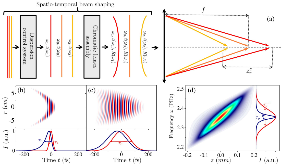
Fig. 1. Generation and properties of CPLC beams. (a) A chromatic linear optical system induces a combination of temporal chirp and frequency-dependent wavefront curvature on an ultrashort beam. When this beam is subsequently focused, its different frequency components have their best focus at different z (longitudinal chromatism). (b) Spatio-temporal field E(\mathbf{r}, t) of the beam prior to focusing in a saturated color scale (negative field in blue, positive in red), in the presence of PFC/LC ( \alpha = 3 \text{ fs/cm}^2 and beam waist w_i = 5 \text{ cm} before focusing, corresponding to \tau_p = \alpha w_i^2 = 75 \text{ fs} ) and in the absence of chirp, for a local pulse duration \tau_F = 25 \text{ fs} . The carrier frequency has been reduced for the sake of readability. Pulse front curvature is clearly observed. (c) Same plot, now in the presence of chirp ( \beta = -6380 \text{ fs}^2 ), i.e., for a CPLC beam. In (b) and (c), the lower panels show the local temporal intensity profile |E(\mathbf{r} = 0, t)|^2 at the center of the beam (red curve), and the spatially integrated temporal intensity profile \int d^2\mathbf{r}|E(\mathbf{r}, t)|^2 (blue curve). These profiles, respectively, have characteristic temporal widths of \tau_F \propto 1/\Delta\omega and \tau_p in the absence of chirp, and \tau_C \propto |\beta|\Delta\omega for strong chirps. (d) On-axis spectrum |E'(z, \omega)|^2 of the focused beam, as a function of the longitudinal coordinate z along the extended Rayleigh length. The right panel compares the local spectrum at z = 0 (blue curve, of characteristic width 1/\tau_p ) with the spatially integrated spectrum \int dz|E'(z, \omega)|^2 (red curve, of characteristic width 1/\tau_F \propto \Delta\omega ).
