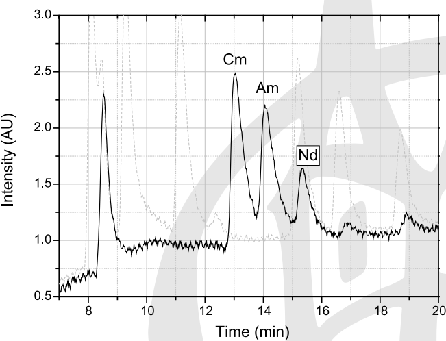
Fig. 6. Chromatogram of Ln separation from an ECRIX-H pellet dissolution solution after treatment (refer to text). The dotted line represents the injection of a surrogate Ln solution. Elution: 0.09–0.23 M HIBA in 20 min in the presence of 0.01 M octanesulfonic acid adjusted to pH 3.7 with NH 3 ; Column: Vydac 201TP5415 150 × 4.6; Elution rate: 1 mL/min; Injection loop: 20 µL; Post-column derivation: PAR 0.05 g/L in 1 M acetic acid + 2 M NH 3 . PAR flow rate: 0.3 mL/min. Detector: HR4000 (Ocean Optics) at 520 nm; Detection cell: Z-flow with 1 cm optical path.
