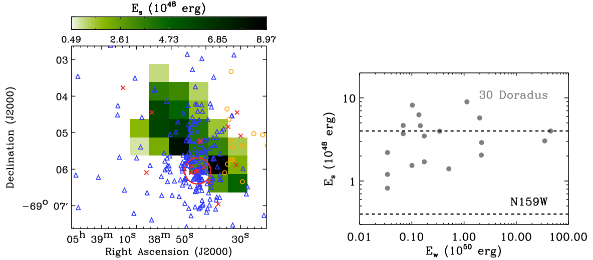
Fig. 18. Left: E_s of the final shock models (shown in Fig. 14) is presented along with \sim 500 stars for which E_w estimates are available ( E_w \geq 10^{50} erg as the red crosses, 10^{49} \text{ erg} \leq E_w < 10^{50} erg as the orange circles, and E_s < 10^{49} erg as the blue triangles; Doran et al. 2013). The location of R136 is also indicated by the red circle. Right: E_s as a function of E_w . The data points for 30 Doradus are shown in gray, while the range of E_s estimated by Lee et al. (2016) for N159W is overlaid as the black dashed line.
