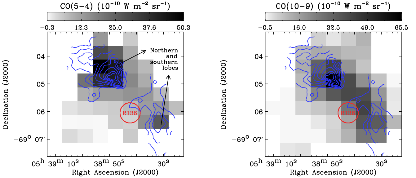
Fig. 4. Comparison between CO ( J = 5-4 and J = 10-9 on the left and right plots) and [C II] 158 \mu\text{m} (blue contours). The PACS [C II] 158 \mu\text{m} data at the original resolution of 12'' are overlaid with levels ranging from 20 to 90% of the peak ( 2.2 \times 10^{-6} \text{ W m}^{-2} \text{ sr}^{-1} ) in steps of 10%. The location of the R136 cluster is indicated by the red circle. We note that the grayscale bar goes below zero simply to show pixels with low intensities.
