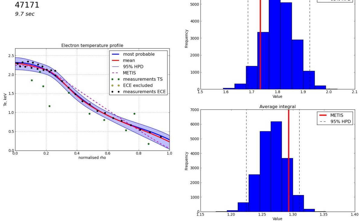
Figure 4: Example of acceptable agreement: electron temperature profile for the shot 47171. Left plot shows the mean (read) profiles and 95% HPD interval (blue area) obtained by Bayesian analysis and METIS result (dashed magenta line); right plots show distribution for the peaking factor and average integral, their 95% HPD interval (range between dashed lines) and the METIS values (red lines).
