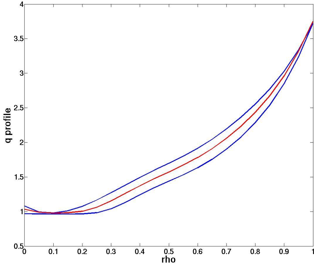
Figure 10: q-profiles at t = 2 s for the Tore Supra shot #47658. The red line corresponds to the METIS simulation with the mean T_e profiles. The two blue lines correspond to the METIS simulations with the highest and lowest possible T_e profiles
