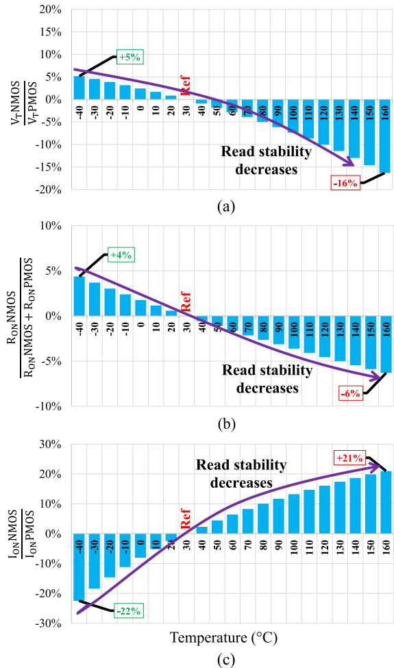
Fig. 8. Temperature effect on (a) V_T , (b) ON-state resistance, and (c) ON-state current of the nMOS and pMOS.
