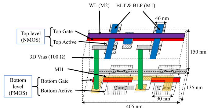
Fig. 9. 3-D picture of the 0.054\text{ }\mu\text{m}^2 4T DL SRAM bitcell in 3-D CoolCube technology [16].
