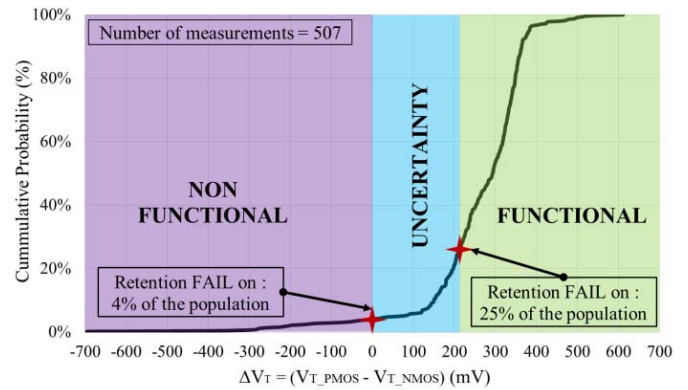
Fig. 12. Data retention validation with silicon data of V_T gap in LETI 14-nm planar FD-SOI technology.
