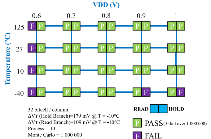
Fig. 18. PASS/FAIL grid for retention and read operations with DBB.
