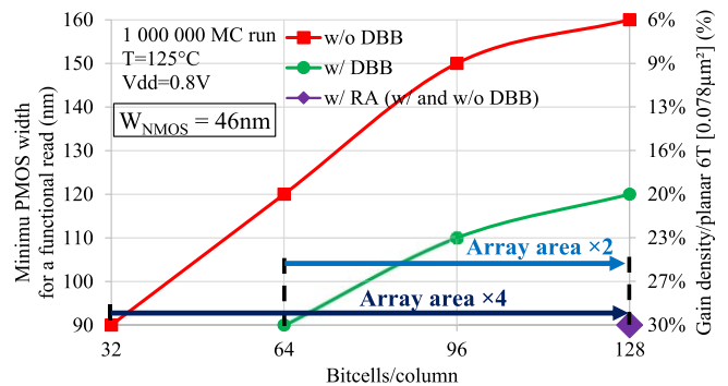
Fig. 22. Minimum pMOS width and gain density with respect to the planar 6T SRAM bitcell ( 0.078\text{ }\mu\text{m}^2 ) versus the number of b/c with and without DBB and with the read assist.
