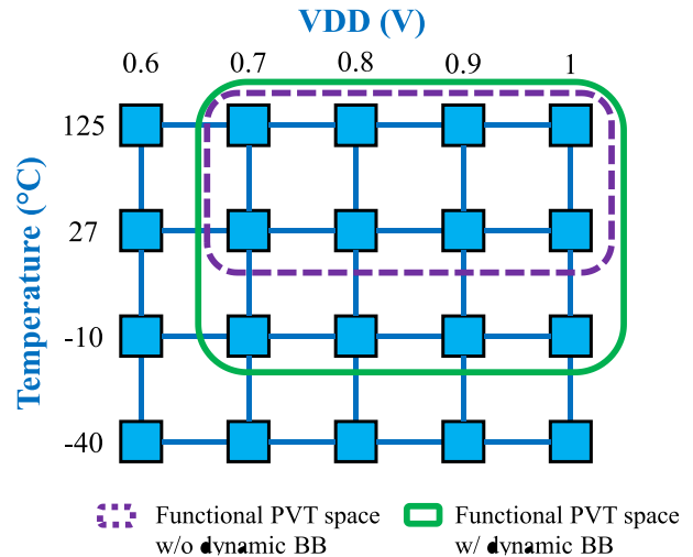
Fig. 19. PVT functional space w/ and w/o DBB.
