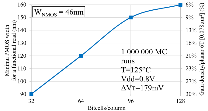
Fig. 14. Minimum pMOS width and gain density with respect to the planar 6T SRAM bitcell ( 0.078 \mu\text{m}^2 ) versus the number of b/c.
