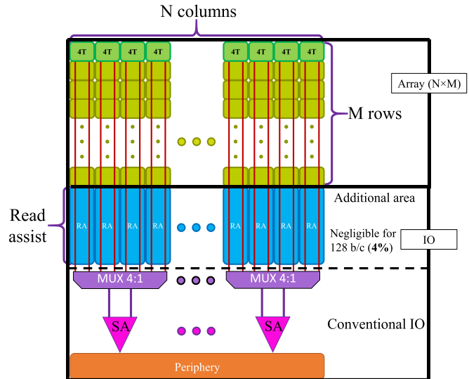
Fig. 21. Placement of the RA on the memory array.
