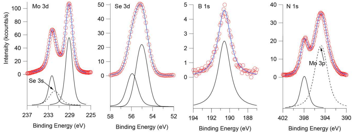
SI Fig. 3. Stoichiometry and thickness estimation. Black lines represent the deconvolution of XPS core levels.
