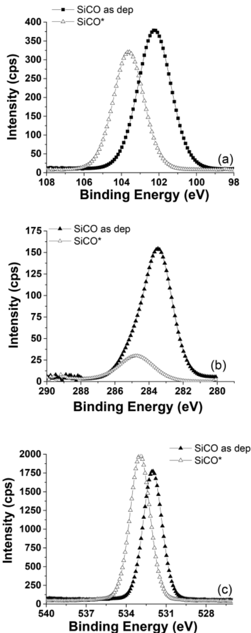
FIG. 6. (a) Si2p, (b) C1s, and (c) O1s spectra recorded by XPS for the as deposited SiCO and SiCO* films.
