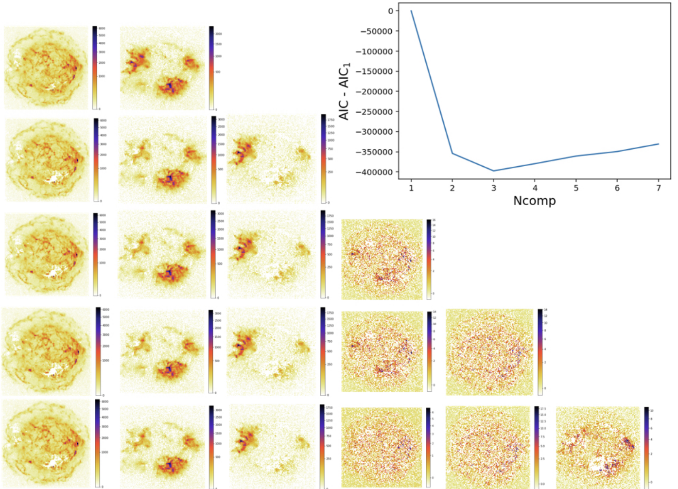
Fig. B.1. Components retrieved by the GMCA applied on Cassiopeia A real data for different values of n . On each line, the retrieved components corresponding to a certain n , beginning with n = 2 on top. On the right, the AIC of the model as a function of this number of components n .
