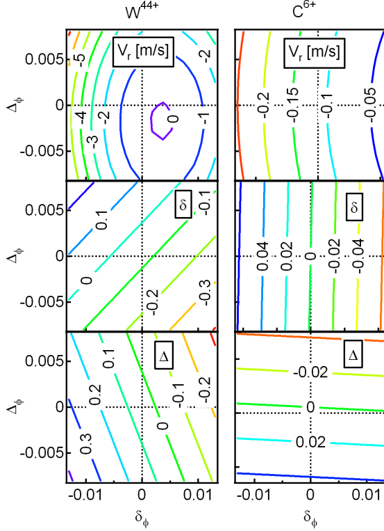
Figure 3. Influence of the asymmetry of the electric potential on W^{44+} (left column) and C^{6+} (right column). From top to bottom: radial velocity, horizontal symmetry, and vertical asymmetry, for the peaked ion density profile case at \sqrt{\psi} = 0.5 .
