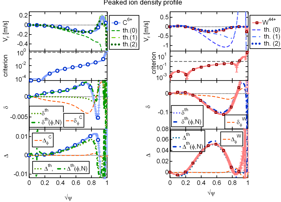
Figure 9. Peaked ion density profile, from top to bottom : profile of the radial particle velocity from the simulation and from analytical estimates, asymmetry criterion from equation (53), horizontal asymmetry and vertical asymmetry from the simulation and from analytical model with and without the contribution of the poloidal asymmetries of the main ion density and of the electrostatic potential, for C^{6+} (left) and W^{44+} (right), with \alpha_\nu = 1 .
