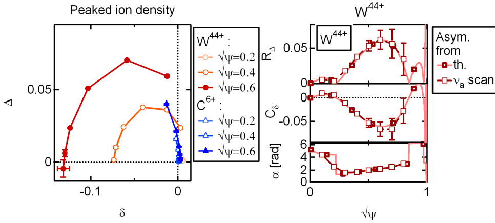
Figure 13. Trajectories of the W^{44+} and C^{6+} poloidal asymmetries at \sqrt{\psi} = 0.2, 0.4 and 0.6 (left), and comparison of the theoretical radius, center and collisional angle at \alpha_\nu = 1 with its geometric determination during the collisionality scan (right), for the peaked ion density profile.
