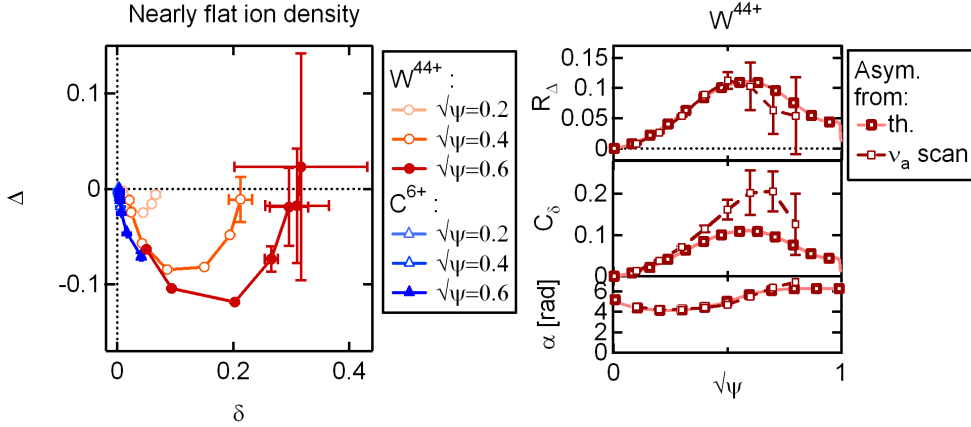
Figure 14. Trajectories of the W^{44+} and C^{6+} poloidal asymmetries at \sqrt{\psi} = 0.2, 0.4 and 0.6 (left), and comparison of the theoretical radius, center and collisional angle at \alpha_\nu = 1 with its geometric determination during the collisionality scan (right), for the nearly flat ion density profile.
