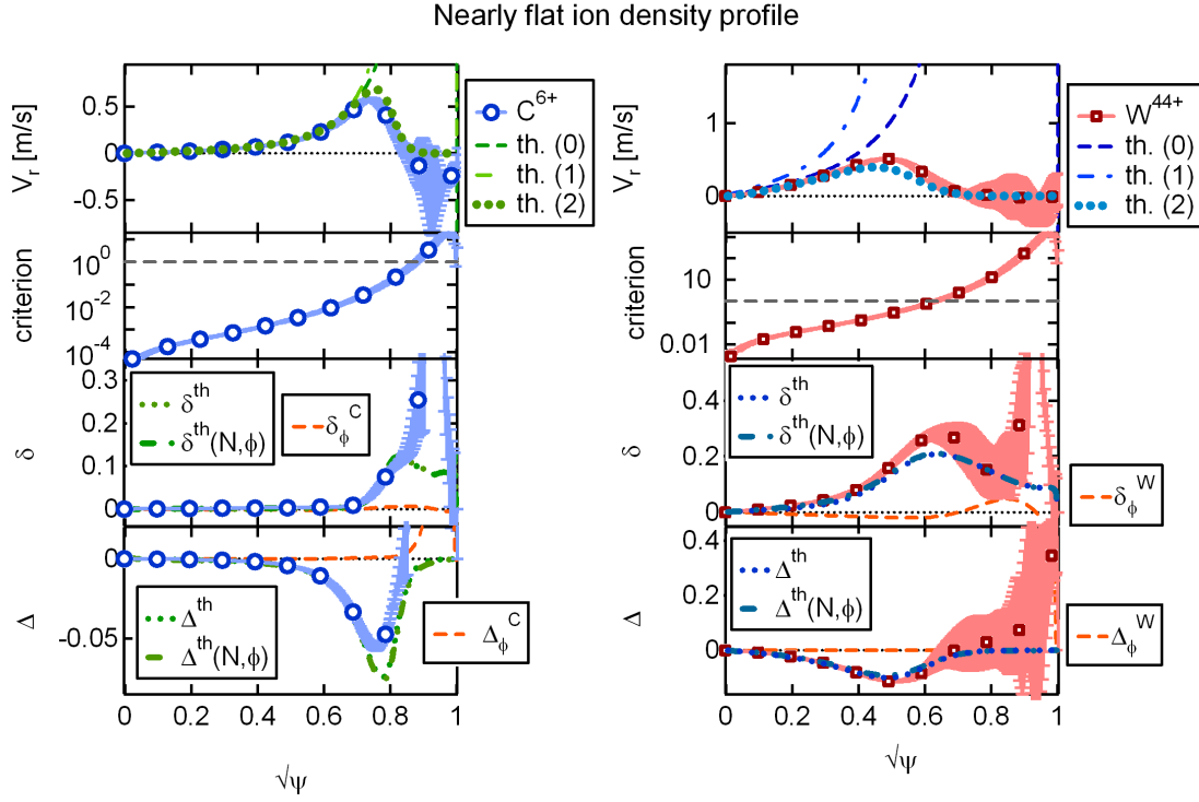
Figure 10. Flat ion density profile, from top to bottom : profile of the radial particle velocity from the simulation and from analytical estimates, asymmetry criterion from equation (53), horizontal asymmetry and vertical asymmetry from the simulation and from analytical model with and without the contribution of the poloidal asymmetries of the main ion density and of the electrostatic potential, for C^{6+} (left) and W^{44+} (right), with \alpha_\nu = 1 .
