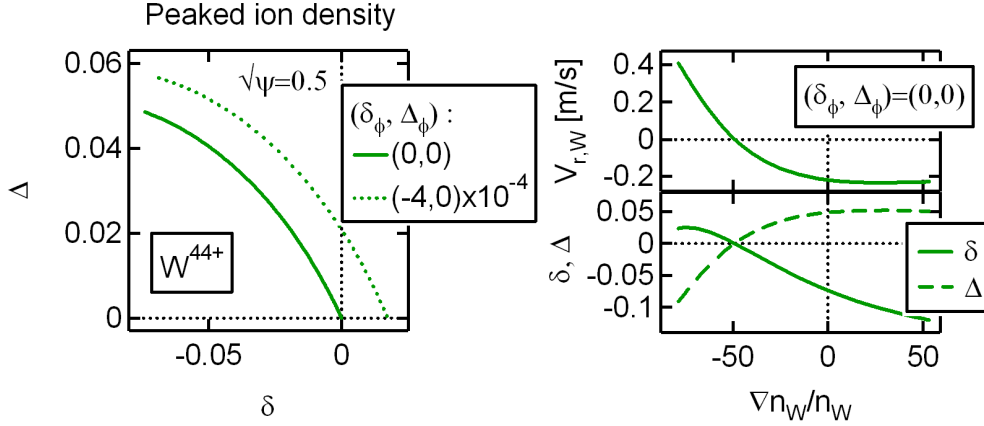
Figure 4. Left : Influence of the asymmetry of the electric potential on the trajectory of the poloidal asymmetry towards steady state, for W^{44+} in the peaked ion density profile case at \sqrt{\psi} = 0.5 . Right: Radial Tungsten velocity (top) and asymmetry ( \delta, \Delta ) as a function of the normalized Tungsten density gradient for (\delta_\phi, \Delta_\phi) = (0, 0) .
