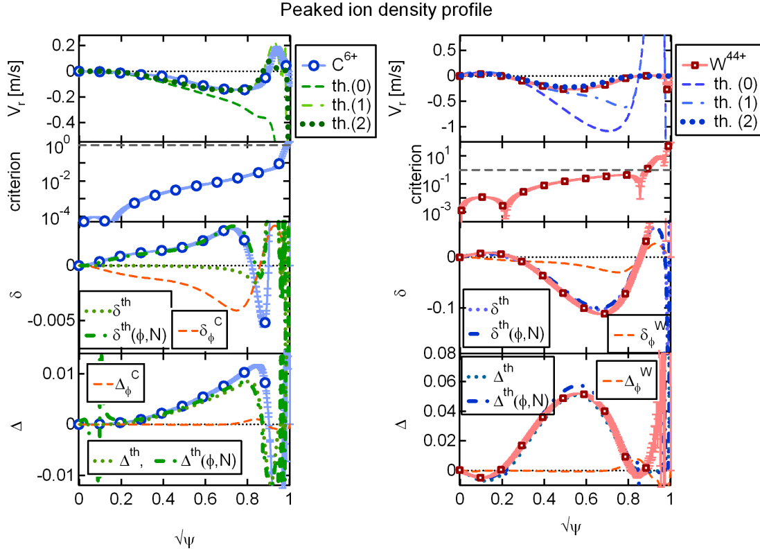
Figure 9. Peaked ion density profile, from top to bottom : profile of the radial particle velocity from the simulation and from analytical estimates, asymmetry criterion from equation (53), horizontal asymmetry and vertical asymmetry from the simulation and from analytical model with and without the contribution of the poloidal asymmetries of the main ion density and of the electrostatic potential, for C^{6+} (left) and W^{44+} (right), with \alpha_\nu = 1 .
