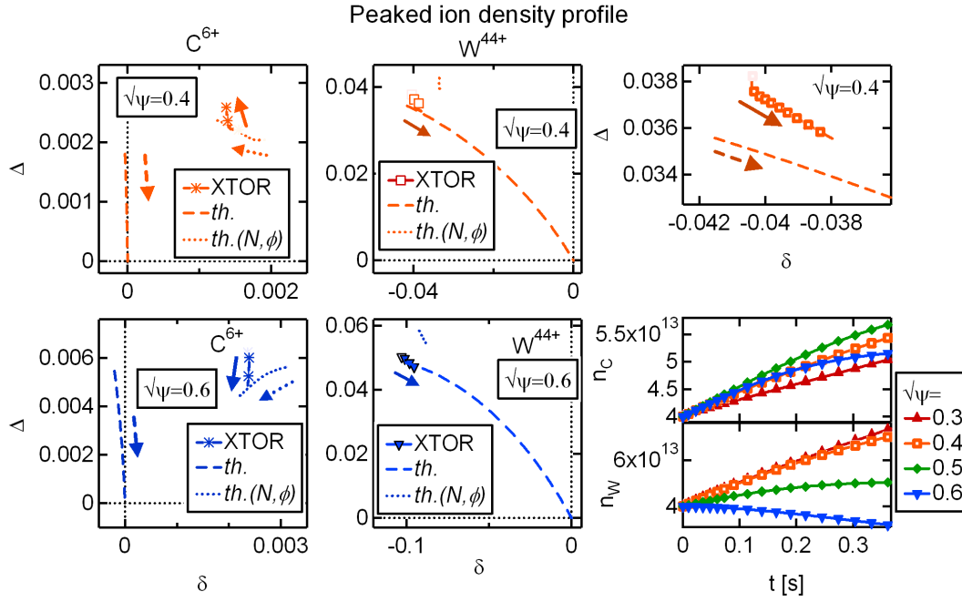
Figure 16. Trajectories in the (\delta, \Delta) plane for C^{6+} (left) and W^{44+} (middle) at \sqrt{\psi} = 0.4 (top) and \sqrt{\psi} = 0.6 (bottom) for the peaked ion density profile. Predictions from the analytical model are shown with a dashed line for (\delta_\phi, \Delta_\phi) = (0, 0) , and with a dotted line when using the measured value of (\delta_\phi, \Delta_\phi) and (\delta_N, \Delta_N) . Right plots: zoom on the W^{44+} trajectory at \sqrt{\psi} = 0.4 (top) and evolution of the Carbon (middle) and Tungsten (bottom) concentrations. Arrows indicate the time evolution.
