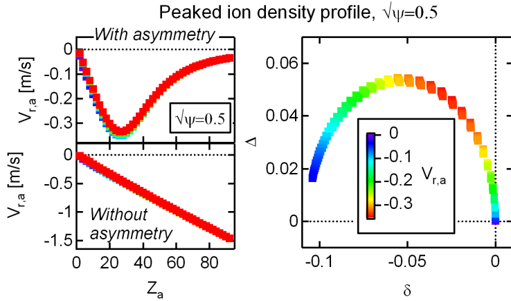
Figure 2. Role of the impurity charge and mass : radial velocity as a function of the ion charge (left plot), with poloidal asymmetry (top) and without (bottom), and vertical asymmetry as a function of horizontal asymmetry (right plot), for the peaked ion density profile described in section 3.2, and for a flat impurity profile. The different points for each impurity charge correspond to different masses.
