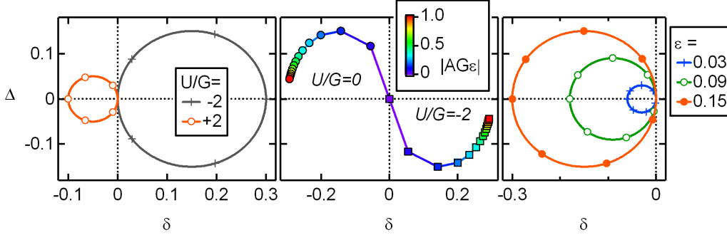
Figure 1. Poloidal asymmetry circle: influence of the equilibrium gradients ( \epsilon = 0.15 , left plot); influence of collisionality ( \epsilon = 0.15 , middle plot); influence of radial position ( U/G = 0 , right plot)
