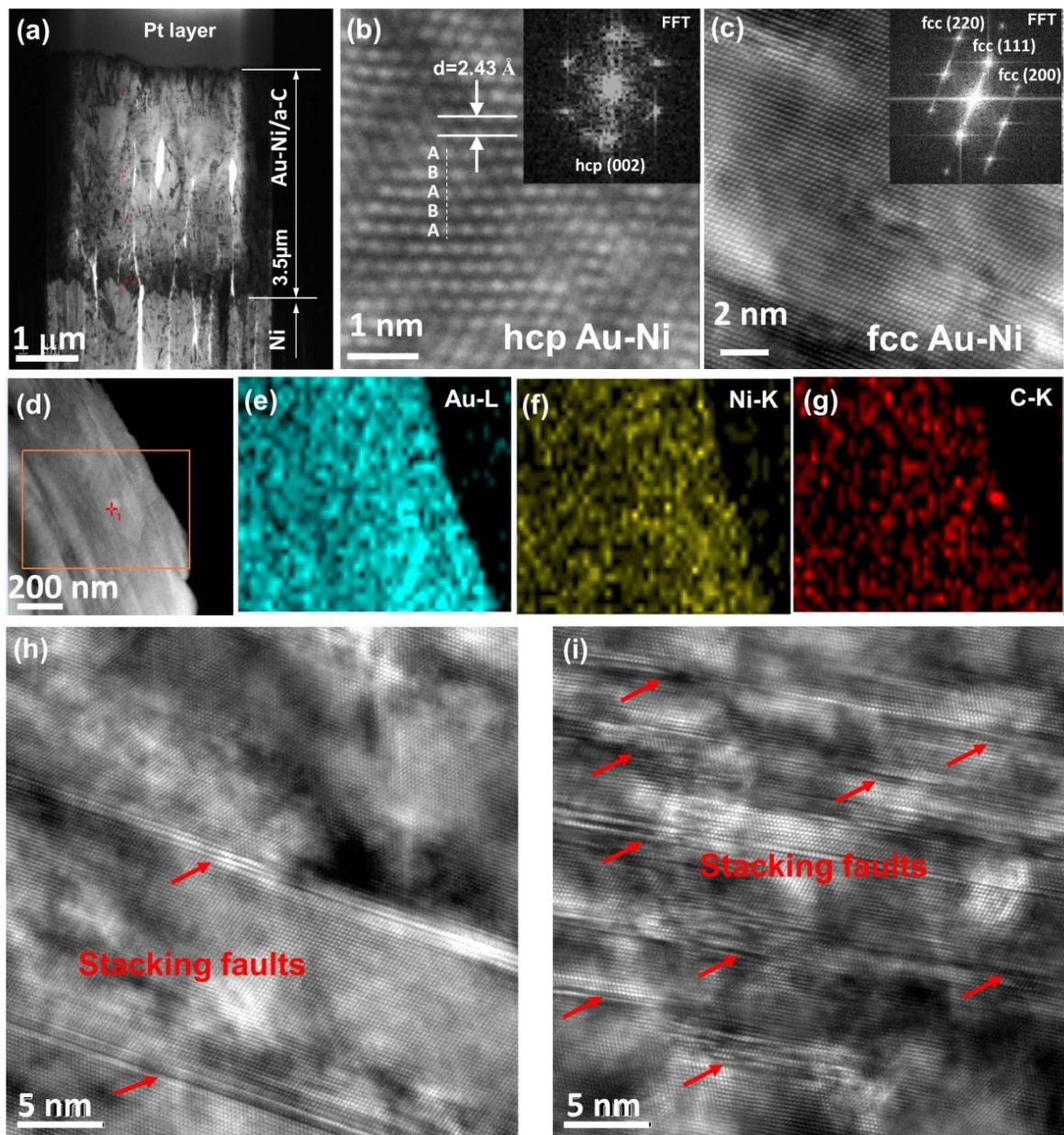
Fig. 5. TEM and EDS mapping images of the Au-Ni/a-C coatings: (a). TEM image shows the entire coating thickness of the Au-Ni/a-C composite coating sample with 1.8 wt.% C, (b). HRTEM of Au-Ni hcp structure and the corresponding FFT pattern of the Au-Ni/a-C composite coating sample with 1.8 wt.% C, (c). HRTEM of the Au-Ni fcc structure and the corresponding FFT pattern of the Au-Ni/a-C composite coating sample with 1.8 wt.% C, (d). The selected EDS mapping area on the Au-Ni/a-C composite coating sample with 1.8 wt.% C, (e-g). EDS mapping of Au, Ni, and C in the square-marked area shown in (d), (g). HRTEM image shows stacking faults of the
