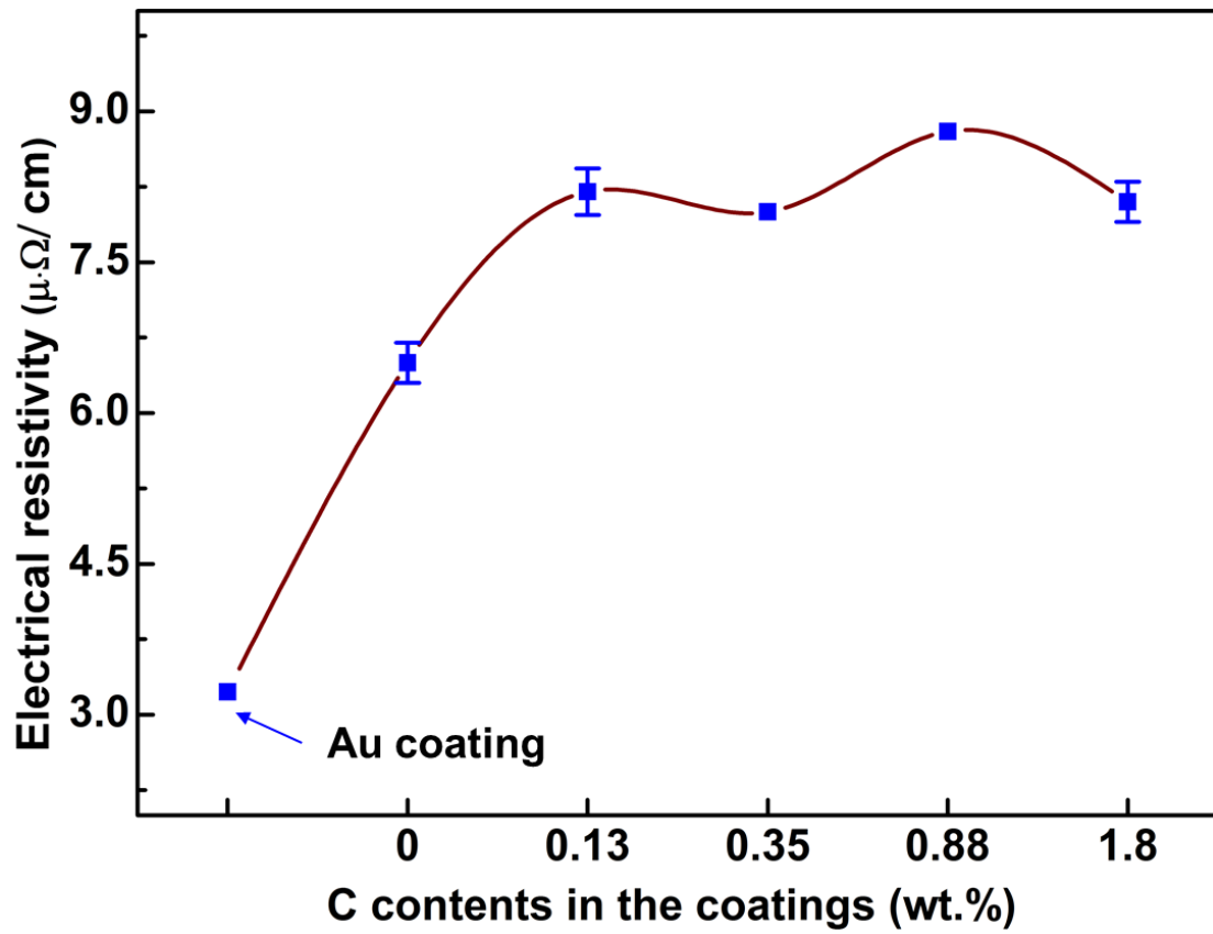
Fig. 10. Electrical resistivities of the deposited coatings.
