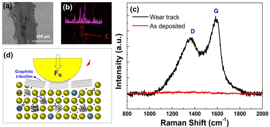
Fig. 12. Wear track characterizations of the Au-Ni/a-C coating with C content of 0.13 wt.%: (a). SEM image of the wear track, (b). EDS mapping of C in the area of (a), (c). Raman spectra in the wear track, (d). Schematic diagram of C lubricant tribofilm generation.
