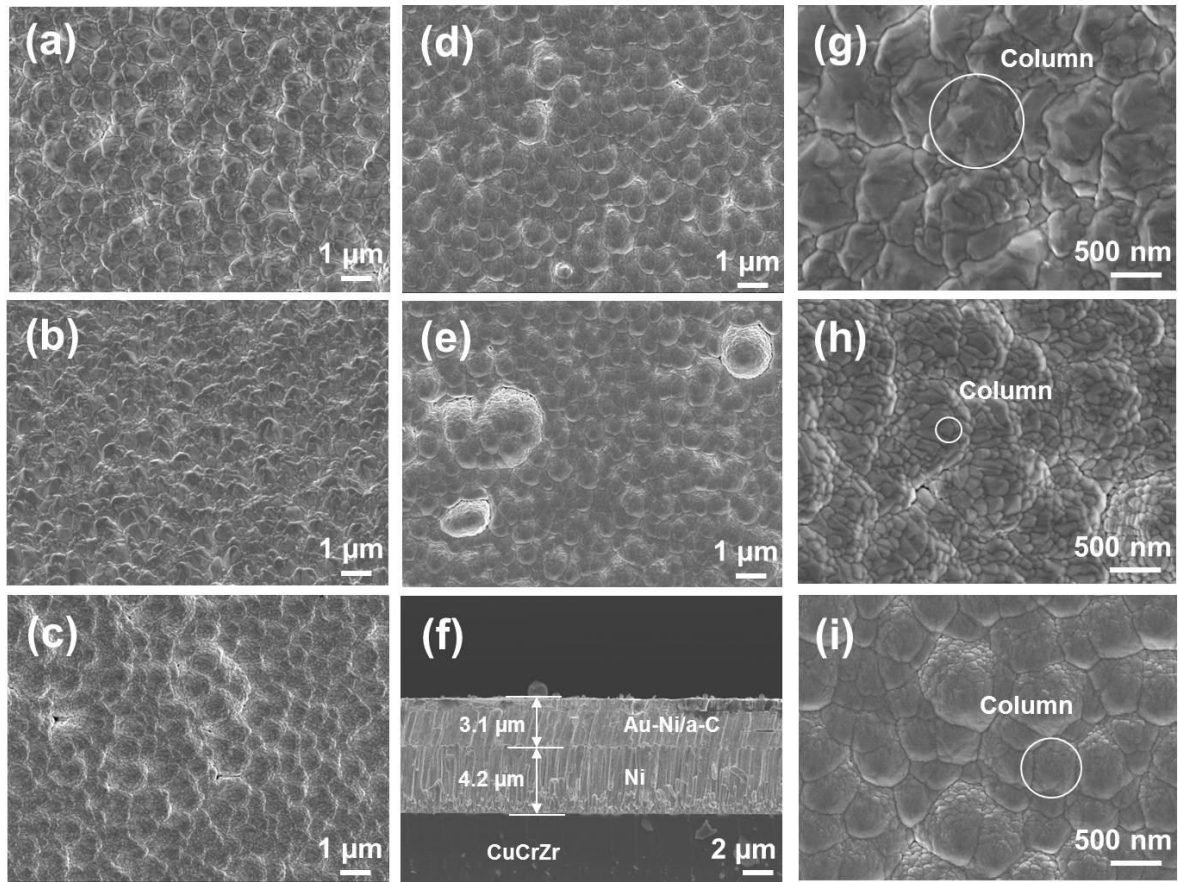
Fig. 2. FESEM images of the coatings deposited at different sputtering powers for the graphite target: (a-e). FESEM images ( \times 10000 ) of the top surfaces of the coatings at 0 W, 100 W, 200 W, 300 W, and 400 W, respectively, (f). FESEM image of the cross-sectional surface of the coating at 400 W, (g- i). FESEM images ( \times 30000 ) of the top surfaces of the coatings at 0 W, 200 W, and 400 W, respectively.
