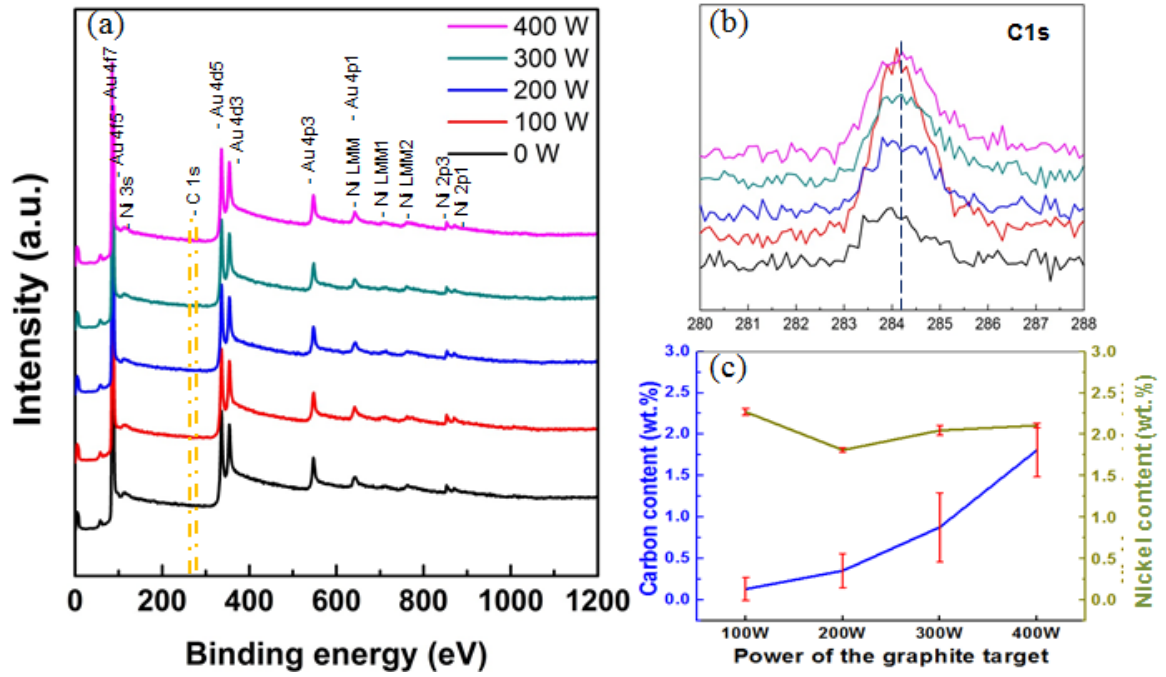
Fig. 3. (a) Full and (b) C1s XPS spectra and (c) compositions of the Au-Ni/a-C composite coatings.
