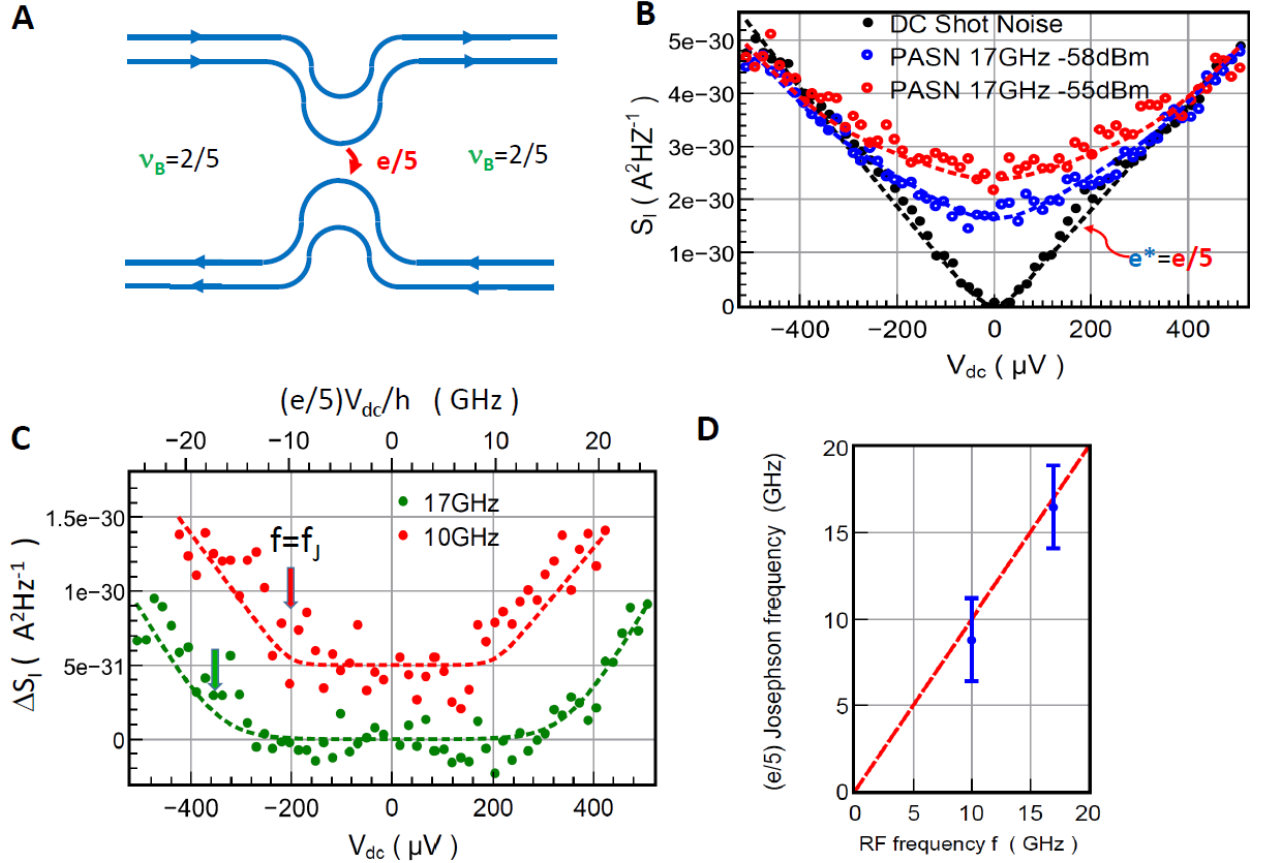
Fig. 3. Josephson relation for the 2/5 FQHE state. (A) Chiral edge schematics: the 2/5 inner edge state is weakly reflected, see point (B) of Fig.1(B). Here backscattered e^*=e/5 carriers contribute to current I_B and shot noise S_I . (B) Raw shot noise measurements: Black dots shows the DC shot noise (i.e. no RF) measured during the 17GHz PASN measurement run. The black dashed line is Eq.(2) using R=0.064 (point (B) of Fig.1(A) ). Blue and red open circles is the PASN for 17GHz -58dBm and -51dBm RF irradiation. Blue and red dashed line curve are comparison using Eq (1) with f_J=(e/5)V_{dc}/h (see Supplementary Information). (C) Excess PASN \Delta S_I . Green and red dots correspond to 17 and 10 GHz. Green and red dashed lines are computed from Eq.(3) using f_J=(e/5)V_{dc}/h . For clarity \Delta S_I(V_{dc}=0) has been subtracted from the excess PASN. (D) Determination of e^* : a best fit of \Delta S_I gives, for each frequency, the threshold voltages V_J=hf/e^* above which \Delta S_I rises. They are plotted in units of (e/5)V_J/h versus f . The dashed line corresponds to e^*=e/5 exactly. According to uncertainties, one finds e^*=e/(5.17 \pm 0.31) .
