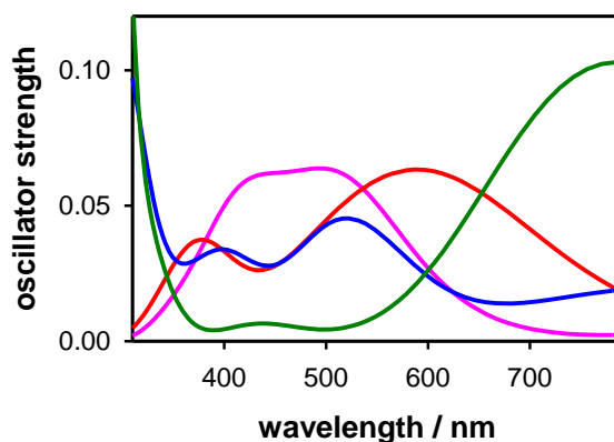
Figure 4. Comparison of the spectra computed for (TG_4T)_4/Na^+ radicals. Pink: radical cation localized on a single guanine 26 ; red: radical cation delocalized over two guanines, 26 green: (G-H_2)^\bullet deprotonated radical; blue (G-H_1)^\bullet deprotonated radical.
