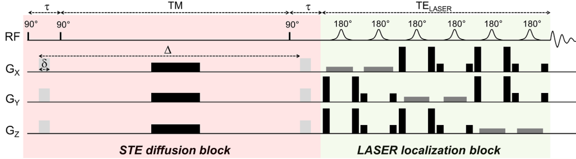
FIG. 1. Outline of the diffusion-weighted STE-LASER sequence. The sequence starts by an STE block, where the 90^\circ are achieved by nonselective 100- \mu s hard pulses. The STE block includes diffusion-weighting gradients (light gray) of duration \delta and separated by \Delta . These diffusion gradients are also used as spoilers to ensure that, when combined with the spoiler inserted during the mixing time (in black), only the stimulated echo is preserved at the end of the block. The sequence is then continued by a LASER localization block, just before acquisition. Because they are isolated from each other (diffusion gradients moment is zero when the LASER block starts), there is no cross-term between diffusion gradients and selection gradients. Total TE = 2\tau + TE_{LASER} .
