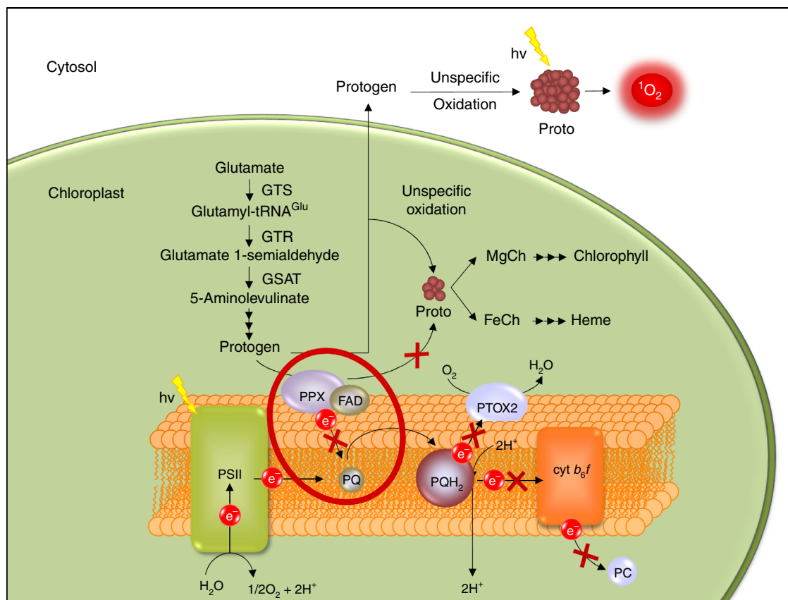
Fig. 4 Schematic representation of a proposed model of the TBS pathway interaction with PET. In normally functioning PET, electrons derived from water are subsequently transferred from photosystem II (PSII) to plastoquinone (PQ) generating its reduced form, plastoquinol (PQH 2 ). PQH 2 is then oxidised by transferring the electrons to cyt b 6 f and by PTOX2. In the ptox2 petB mutant, the PQ pool is almost completely reduced 9 , as depicted by the greater PQH 2 oval (PQ«PQH 2 ). In such conditions, PPX cannot transfer the electrons derived from Protogen to PQ. FAD cofactor present in PPX is proposed to mediate in electron transfer from PPX to PQ. Thus, lack of the oxidised plastoquinone (PQ) leads to a dysfunction or a complete blockage of the PPX function. This in turn prevents synthesis of Proto in a controlled fashion. Subsequently, Protogen is unspecifically oxidised in the chloroplast and after sequestration in the cytosol, leading to the formation of Proto, which is inaccessible for MgCh and FeCh. Ultimately, accumulating Proto leaks out of the chloroplast and outside of the cell, which is observed as the brownish precipitate in the media. However, a small portion of the Proto formed in the chloroplast may be still available for the enzymes subsequently leading to biosynthesis of chlorophyll and heme
