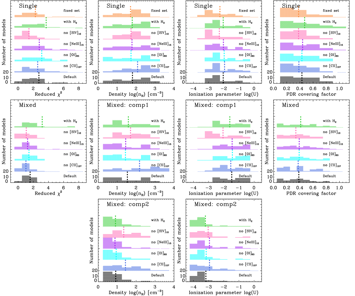
Fig. 6. Sensitivity of the model results to the fitted lines. We show histograms of the reduced \chi^2 ( \chi^2_{\nu} ) and best-fitting parameters ( n_{\text{H}} , \log U , \text{cov}_{\text{PDR}} ) for the entire sample of galaxies. The results from the default grid of models and the default set of lines are in black, and the results are in color if the set of fitted lines is changed, that is, when one spectral line is excluded or when the \text{H}_2 lines included or when we consider a small, fixed set of lines to fit ( [\text{Ne III}]_{15} , [\text{O III}]_{88} , [\text{C II}]_{157} , and L_{\text{TIR}} ). The vertical dotted lines indicate the mean values. Each histogram is offset vertically by a value of 20. See Sect. 5.1 for details.
