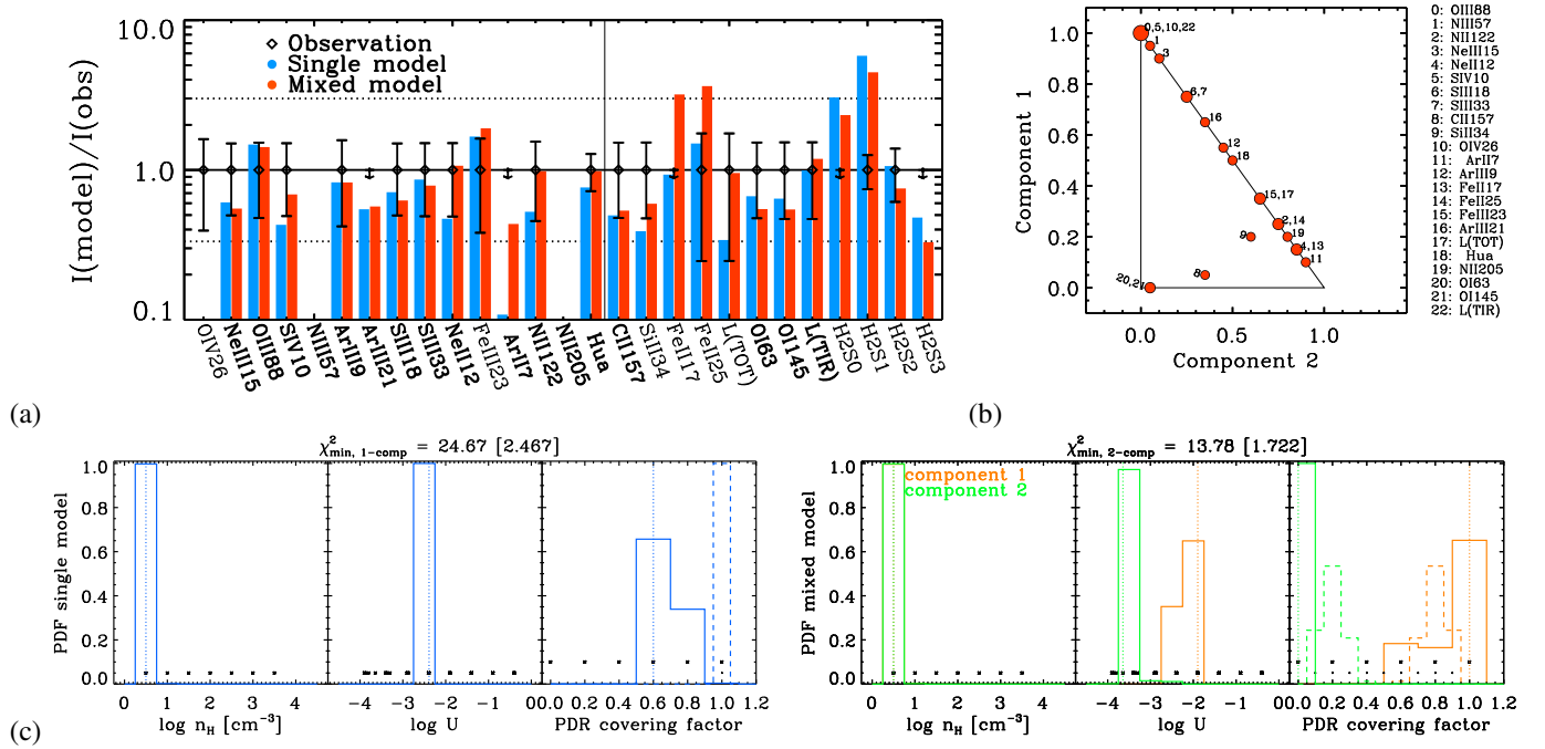
Fig. D.19. Results for NGC 1140. Panel a : comparison of the observed (losange) and predicted intensities for our best-fitting single (blue bar) and mixed (red bar) H II region+PDR models. Lines are sorted by decreasing energy. The fitted lines have labels in boldface. Panel b : for mixed models: respective contributions from component #1 and component #2 to the line prediction. For PDR lines ([C II], [O I], and [Si II]), only the contribution from the ionized gas is shown; the PDR contribution is one minus the sum of the contributions from the plot. Contributions are expected to be dominated by one or the other component if their model parameters are noticeably different. Panel c : probability density functions of the model parameters ( n_{\text{H}} , U , \text{cov}_{\text{PDR}} /scaling factor) for single ( left panel ) and mixed ( right panel ) models. The scaling factor corresponds to the proportion in which we combine two models in the mixed model case. It is equal to unity otherwise. It is shown with dashed lines in the same panels as the PDR covering factor. Vertical dotted lines show values of the best-fitting model. Black asterisks show the range and step of values of the grid parameters.
