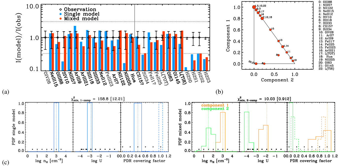
Fig. D.3. Results for Haro 11. Panel a: comparison of the observed (losange) and predicted intensities for our best-fitting single (blue bar) and mixed (red bar) H II region+PDR models. Lines are sorted by decreasing energy. The fitted lines have labels in boldface. Panel b: for mixed models: respective contributions from component #1 and component #2 to the line prediction. For PDR lines ([C II], [O I], and [Si II]), only the contribution from the ionized gas is shown; the PDR contribution is one minus the sum of the contributions from the plot. Contributions are expected to be dominated by one or the other component if their model parameters are noticeably different. Panel c: probability density functions of the model parameters ( n_H , U , \text{cov}_{\text{PDR}} /scaling factor) for single ( left panel ) and mixed ( right panel ) models. The scaling factor corresponds to the proportion in which we combine two models in the mixed model case. It is equal to unity otherwise. It is shown with dashed lines in the same panels as the PDR covering factor. Vertical dotted lines show values of the best-fitting model. Black asterisks show the range and step of values of the grid parameters.
