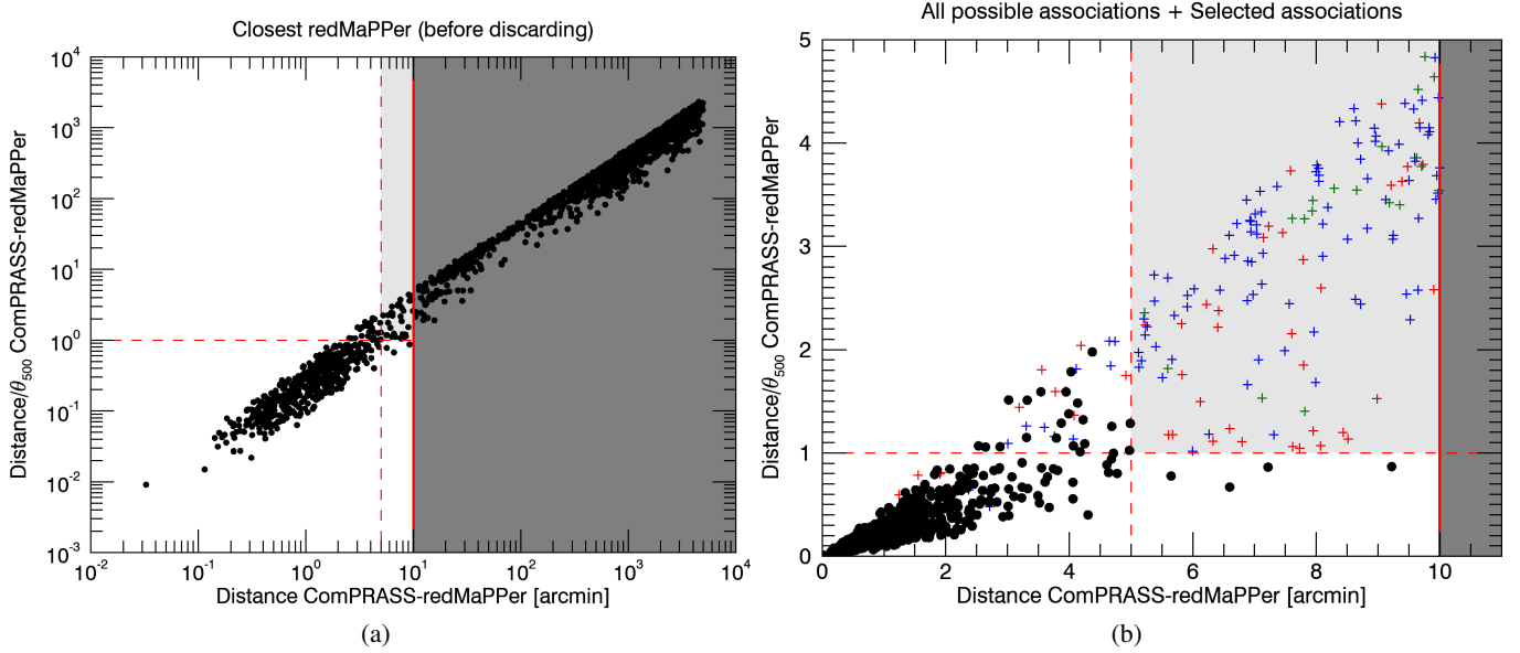
Fig. 8. Positional criteria for matching ComPRASS candidates to redMaPPer clusters. Panel a: closest redMaPPer cluster to each ComPRASS candidate. Panel b: all the possible redMaPPer counterparts within 10 arcmin of each ComPRASS candidate. Red, blue, and green symbols represent the closest, second-closest, and third-closest counterpart (if it exists), respectively. The black circles identify the pairs that are finally selected. The blue and red coloured crosses in the d < 5 region correspond to associations that satisfy the positional criteria, but that are finally discarded by the richness cut.
