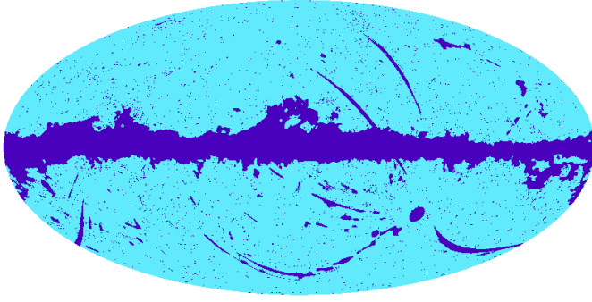
Fig. 1. Mask applied to the second phase detections. This results from the combination of the SZ mask and the X-ray exposure time mask. The dark-blue areas are masked, the light-blue area is the final footprint, which accounts for 80.96% of the sky. The electronic version of this mask is available at the CDS.
