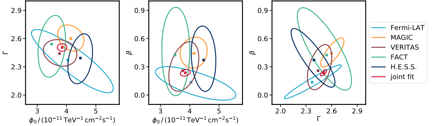
Fig. 3. Likelihood contours corresponding to 68% probability content for the fitted spectral parameters (\phi_0, \Gamma, \beta) , for the likelihood in Eq. (1). Results from the individual instruments and from the joint-fit are displayed.
