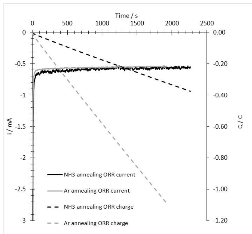
Figure A2. Examples of ORR chronoamperometry measurements (and corresponding charge) performed on an NH 3 annealed electrode sample (black lines) and an Ar annealed electrode sample (grey lines). The loading for the NH 3 annealed electrodes sample is 2.29 mg·cm -2 , and the loading for the Ar annealed electrode sample is 3.82 mg·cm -2 . The selectivities calculated for both of the electrodes are shown in Figure 6.
