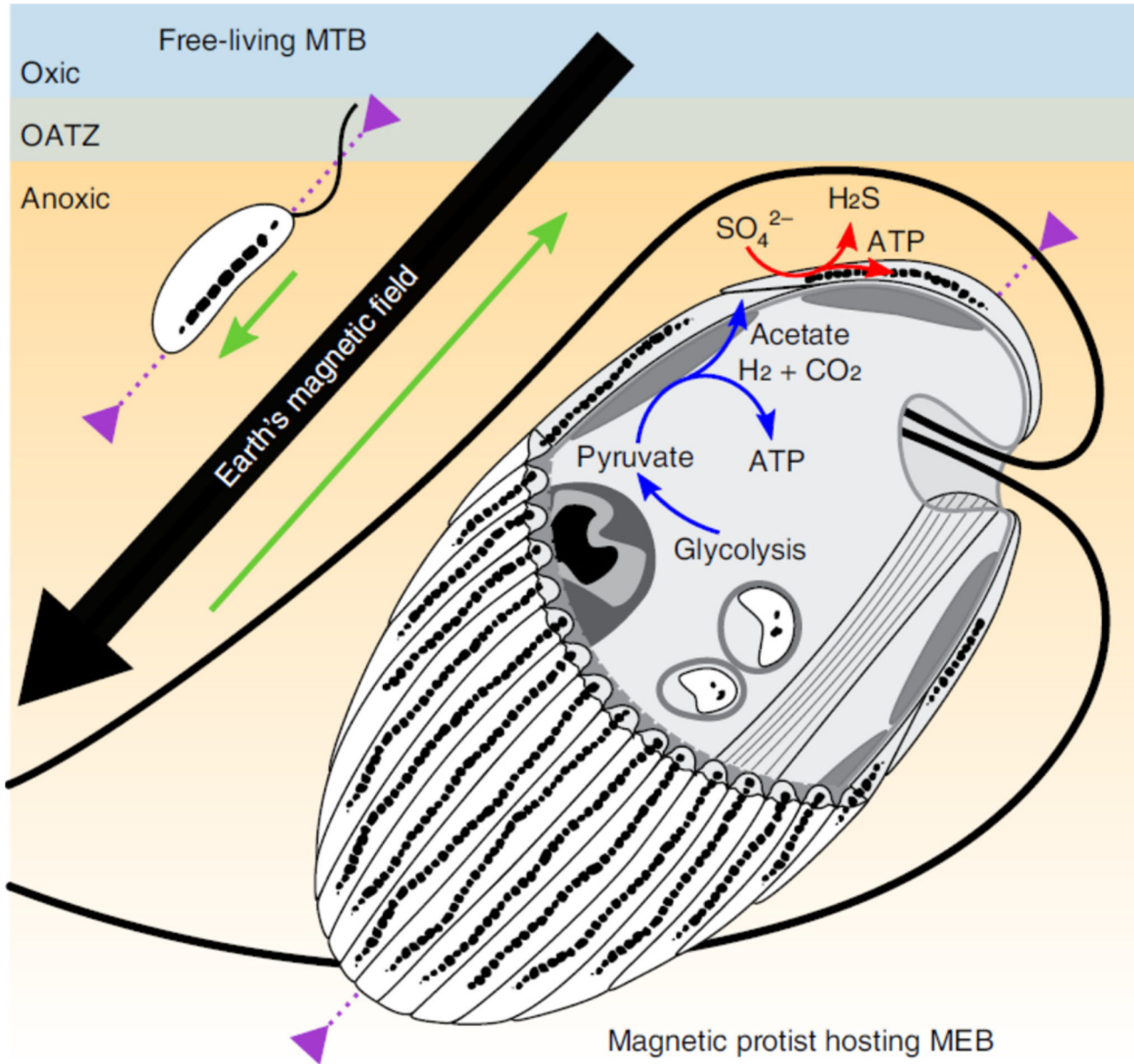
Fig. 4. Schematic illustration of the magnetotactic consortium showing the magnetotactic behaviour in the Northern Hemisphere and the syntrophic interactions between partners. The green arrows show the anterior–posterior orientation of the organisms, which is parallel and antiparallel to the Earth’s magnetic field lines for the freeliving magnetotactic bacteria (MTB) and the consortium protist-MEB, respectively. The purple arrows show the organism’s motility zone in the sediments. The ATP synthesis by the hydrogenosomes in the protist is symbolized by the blue arrows. Molecular hydrogen, acetate and carbon dioxide are products that could be transported through the plasma and used by the MEB as sources of energy and carbon. The red arrows show the dissimilatory sulfate reduction by MEB,
