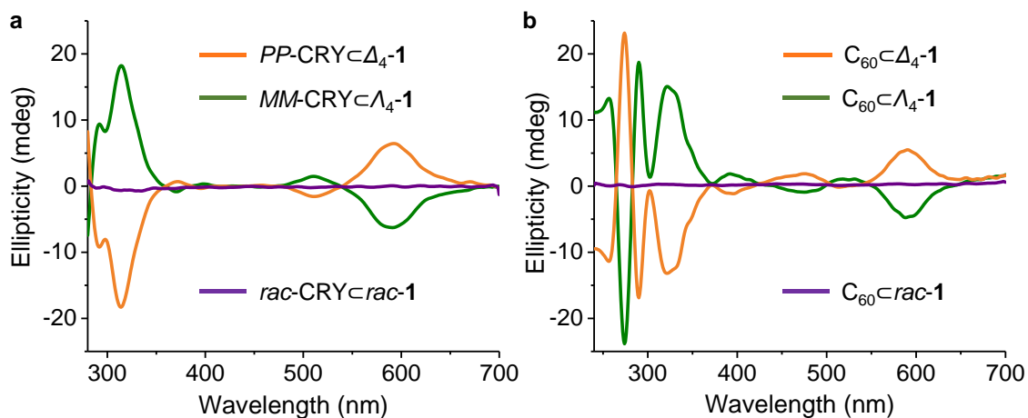
Figure 5. (a) CD spectra of PP\text{-CRY} \subset \Delta_4\text{-1} (orange), MM\text{-CRY} \subset \Lambda_4\text{-1} (green) and rac\text{-CRY} \subset rac\text{-1} (purple). (b) CD spectra of C_{60} \subset \Delta_4\text{-1} (orange), C_{60} \subset \Lambda_4\text{-1} (green) and C_{60} \subset rac\text{-1} (purple), formed following CRY guest displacement.
