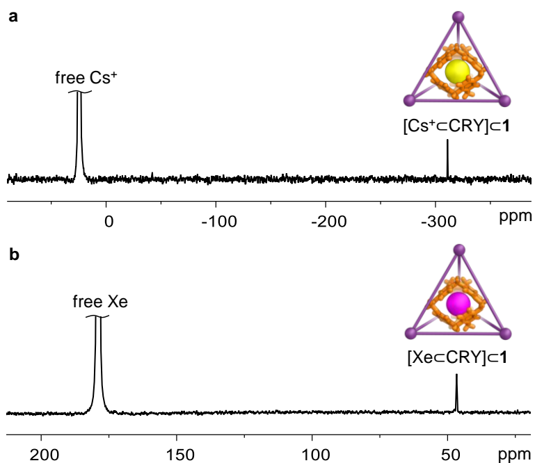
Figure 3. (a) ^{133}\text{Cs} NMR ( \text{CD}_3\text{CN} , 66 MHz, 60 °C) spectrum of CRY \subset \mathbf{1} in the presence of excess \text{Cs}^+ . (b) ^{129}\text{Xe} NMR ( \text{CD}_3\text{CN} , 138 MHz, 25 °C) spectrum of CRY \subset \mathbf{1} in the presence of excess Xe.
