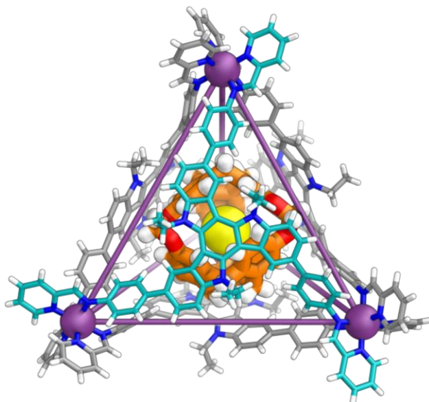
Figure 2. Crystal structure of [Cs + ⊂CRY]⊂1 illustrating the [Cs + ⊂PP-CRY]⊂Δ 4 -1 enantiomer. The bound Cs + , CRY and the front triazatruxene face are colored yellow, orange and cyan, respectively. Disorder, unbound counterions, and solvent of crystallization are omitted for clarity and only one of the two crystallographically independent complexes is shown.
