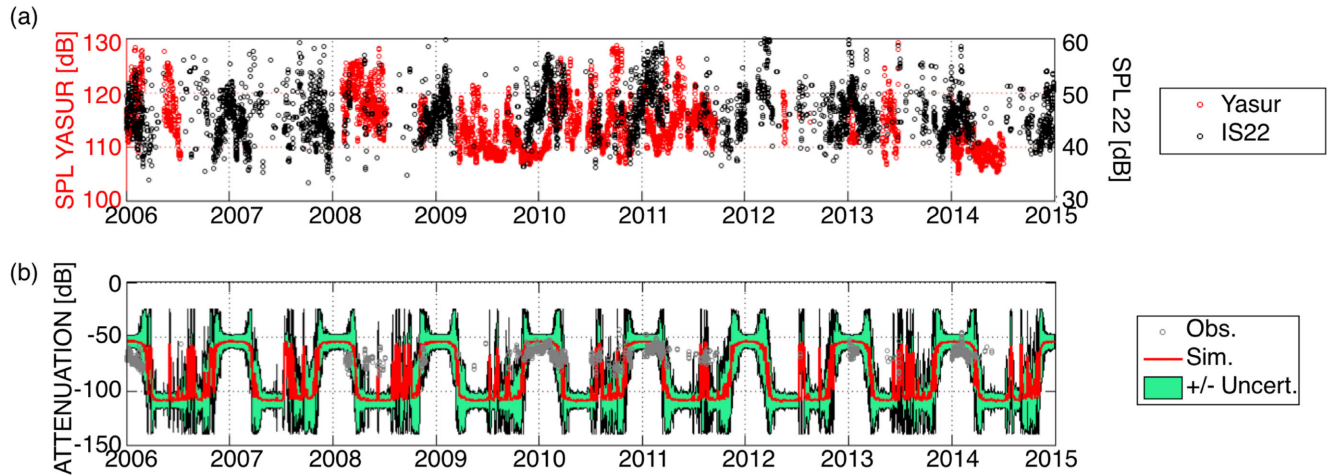
Figure 6. Simulated detection capability at IS22 using Mt. Yasur infrasound signals observed at Melkem (2006–2015). (a) Comparison between the sound pressure level (SPL) measured at Mt. Yasur (in red dots, corrected for spreading to 1 km) and IS22 (in black dots). During austral summer, the downwind periods favour long-range propagation of signals from Mt. Yasur, with a constant attenuation of -70 dB. (b) Comparison between the simulated wave attenuation (red curve) and the one derived from near- and far-field observations (grey dots). Simulations are carried out at the dominant frequency of the recorded signals (2 Hz). Green areas delimit the 95 per cent confidence interval of the predicted attenuation when including 10 \text{ m s}^{-1} wind speed random perturbations at stratospheric altitudes. During the equinoxes, larger detection periods are noted when incorporating these uncertainties.
