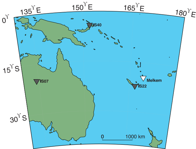
Figure 5. Geographical locations of stations used in this study. Grey and white reverse triangles indicate IMS and national arrays, respectively. Melkem station is located less than 5 km from the Mt. Yasur volcano.
