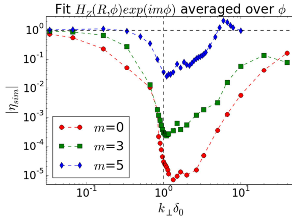
Figure 11: Numerical reflection coefficient \eta_{sim} , vs k_{\perp}\delta_0 , for varying azimuthal number. Vertical dashed line k_{\perp}\delta_0=1 . Simulations using parameters of series #1 in table 2, R_0=0.5m , \delta R=16mm , unbounded stretching function (IV.4) and scan of \delta_0 . Element size 5mm over whole simulation domain.
