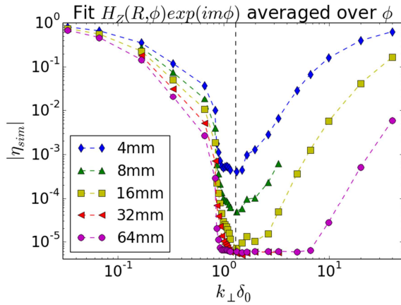
Figure 10: Numerical reflection coefficient \eta_{\text{sim}} , vs k_{\perp}\delta_0 , for several PML depths \delta R . Vertical dashed line k_{\perp}\delta_0=1.3 . Simulations using parameters of series #1 in table 2, R_0=0.5\text{m} , unbounded stretching function (IV.4) and scan of \delta_0 . Element size 5mm over whole simulation domain.
