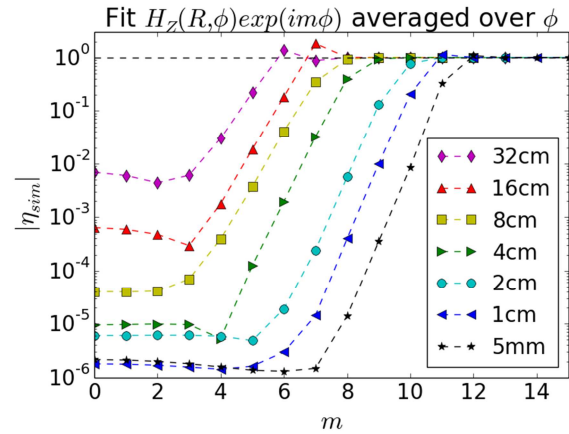
Figure 12: Numerical reflection coefficient \eta_{sim} , vs azimuthal number m . Simulations using parameters of series #1 in table 2, \delta R=50cm and unbounded stretching function (IV.4) with k_{\perp}\delta_0=1.5 . Element size 5mm in main simulation domain, various mesh size in the PML.
