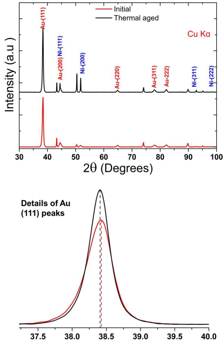
Fig. 2 XRD pattern of Au-Ni coating on CuCrZr (original and thermally aged)
