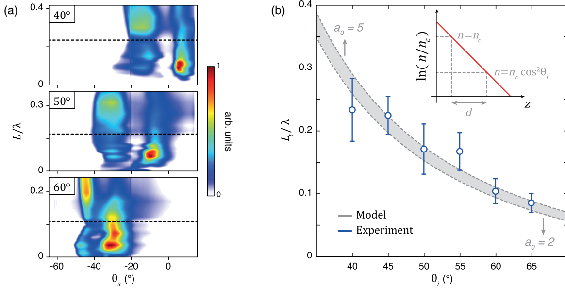
FIG. 12. Effect of the laser incidence angle on the laser-plasma coupling. Panel (a) shows the evolutions with L of the high-energy electron beam angular profile in the incidence plane, measured for three different incidence angles, for a laser field amplitude a_0 \approx 3.5 . For each angle, L is measured experimentally using the SDI technique. The value L_t^e where a transition occurs is clearly observed to decrease with \theta_i . The measured evolution of L_t^e with \theta_i is plotted in (b), where it is compared to the simple model described in the text. The predictions of this model are shown for a range of laser amplitudes 2 \leq a_0 \leq 5 , to account for the experimental uncertainty on this amplitude. These predictions are very close to the high-amplitude limit given by Eq. (1).
