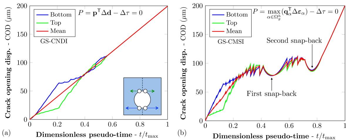
Figure 16: Perforated plate – Pseudo-time evolutions of \text{COD}_{\text{top}} , \text{COD}_{\text{bottom}} and \text{COD}_{\text{mean}} obtained through the GS-CNDI (a) and GS-CMSI (b) formulations
