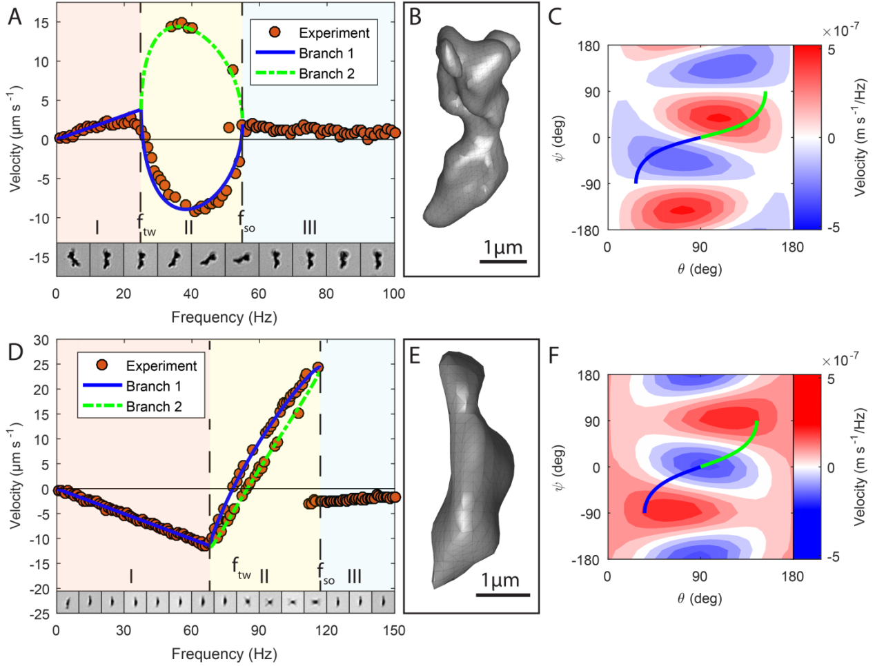
Figure 1. Velocity-frequency-relationship. The measured velocity (red dots) dependent on the applied frequency of the actuating magnetic field is shown in a panel A and D for propeller 1 and 2 respectively. The theoretic fit on those data points is shown in blue (solid line) and green (dashed line), which also describes the observed branching (corresponding to different propeller configuration at the respective frequencies). The 3D-reconstruction of the propellers is depicted in panel B and E . To visualize the change in propeller configuration to the horizontal axis of rotation dependent on the frequency, microscope images are shown in the measured frequency regime for one respective branch (Panel A and D on the bottom). The most left image corresponds to the orientation for a constant field in between the measurements. Both propellers show a reversal of the velocity direction in the first branch (blue), when increasing the frequency: after a linear tumble regime ( I , swimming in one direction) until f_{tw} , a non-linear wobbling regime ( II ) happens up to the step-out frequency f_{so} ( III ). During the wobbling, the long axis of the propeller starts to tilt more and more towards the horizontal axis of rotation and at a certain frequency, the propeller velocity reverses its sign – the propeller swims in the opposing direction. The respective velocity landscapes are shown in C and F as contour plots (red for positive velocities, blue for negative ones and white for zero). They reflect the velocity possibilities (in \text{m s}^{-1}/\text{Hz} ) of the respective propeller shape. The green and blue lines are again the branches, since the propellers are restricted to certain rotation axes for increasing frequency. The rotational similarity of propeller 2 is reflected in its velocity landscape. As a result, the branches pass similar values for increasing frequency (in contrast to propeller 1).
