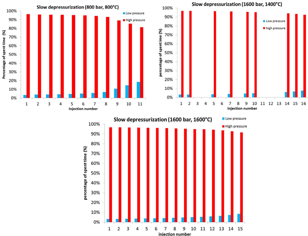
Fig. 28. Residence time in the high and low pressure regions.
