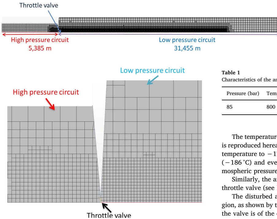
Fig. 13. Zoom on the throttle valve region.
