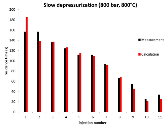
Fig. 25. Analytical results for test 1.
