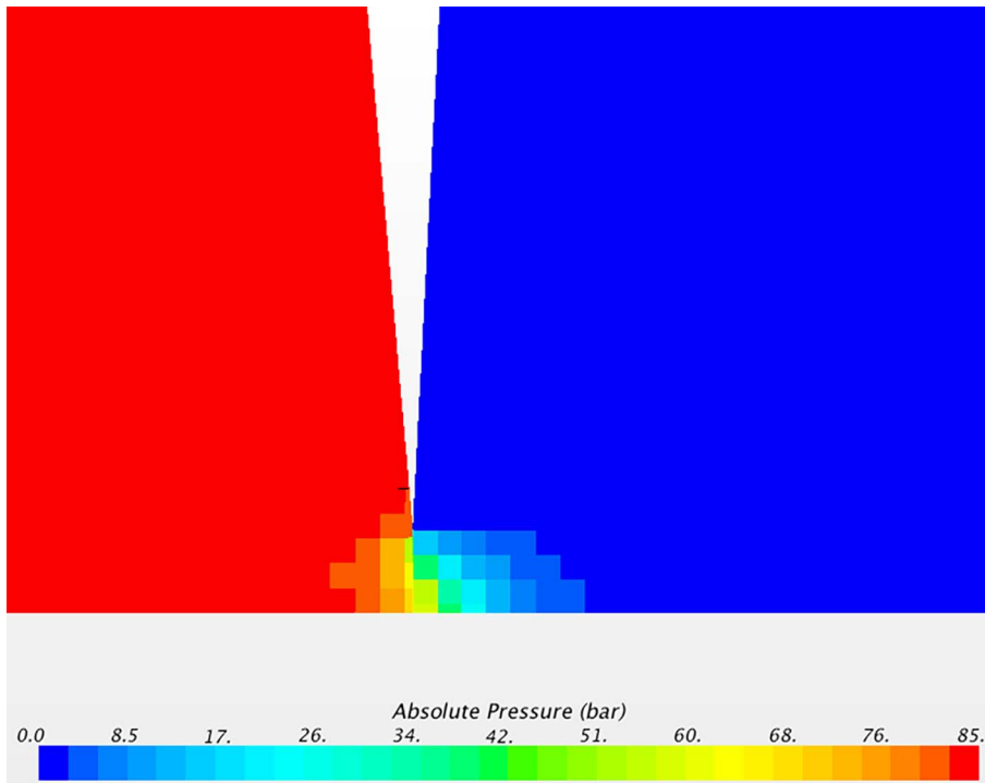
Fig. 15. Zoom on the pressure near the throttle valve.
