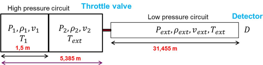
Fig. 24. Decomposition of the argon flow field into three flow regions.
