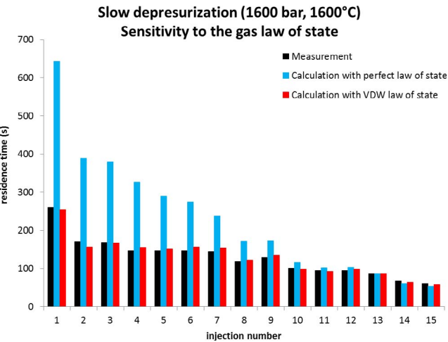
Fig. 30. Impact of the equation of state on the residence time.
