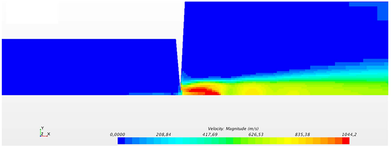
Fig. 17. Zoom on the velocity for the transit of the throttle valve.
