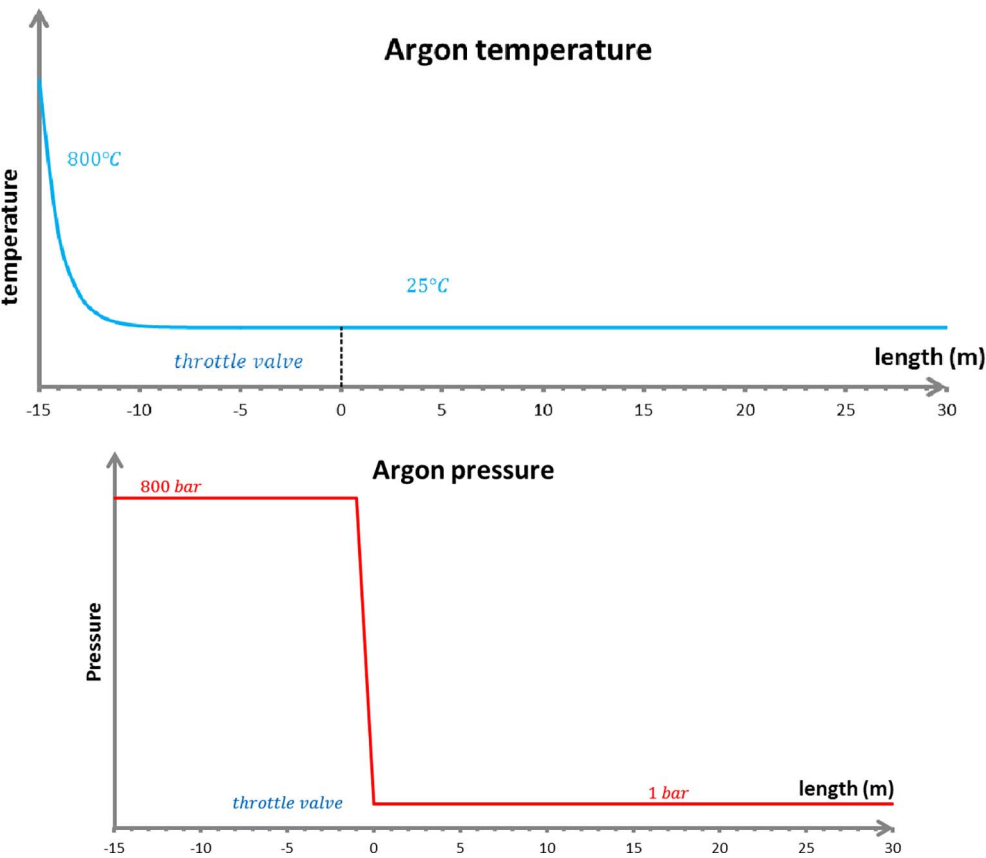
Fig. 23. Evolution of the argon temperature and pressure versus the z axis.
