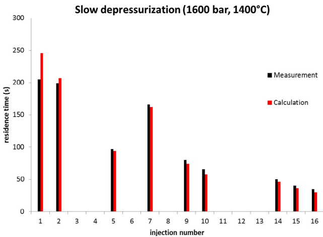
Fig. 26. Analytical results for test 2.
