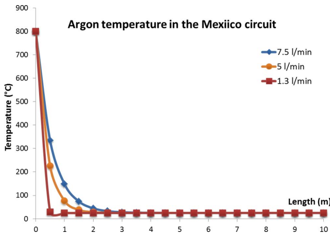
Fig. 22. Evolution of the temperature along the loop according to the flow.
