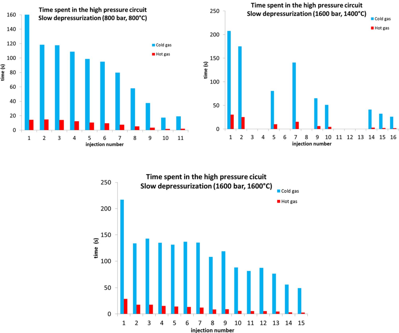
Fig. 29. Time spent the high pressure region.
