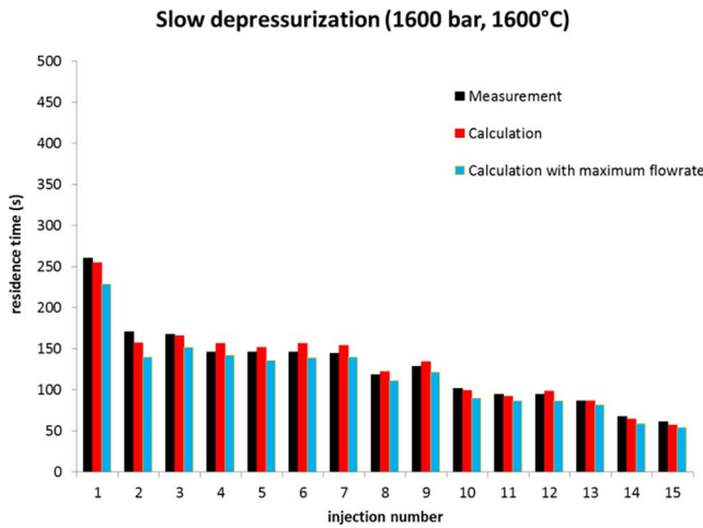
Fig. 32. Residence time: sensitivity to uncertainty in the flowrate.
