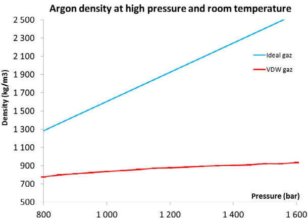
Fig. 31. argon density at high pressure and room temperature.
