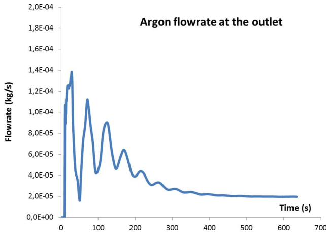
Fig. 21. Mass flowrate downstream of the valve.
