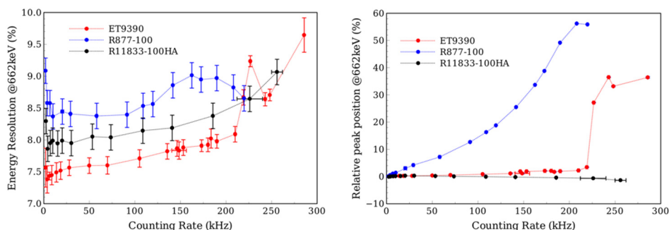
Fig. 4. (left) Energy resolution and (right) relative peak position at 662 keV as a function of the counting rate for the three PMTs under study.
