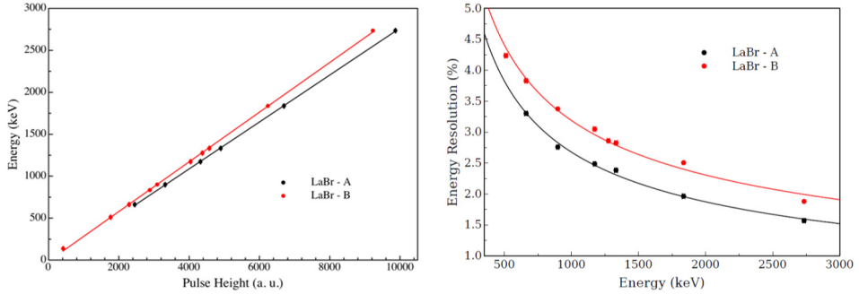
Fig. 5. (left) Energy calibrations and (right) energy resolution curves for the two 3 in \times 3 in LaBr 3 :Ce scintillators.
