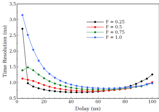
Fig. 7. Time resolution (FWHM) of the LaBr 3 :Ce system as a function of the DCFD delay for different values of fraction.
