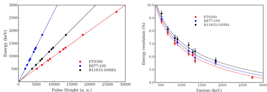
Fig. 3. (left) Energy calibration and (right) resolution curves for the three PMTs under study.
