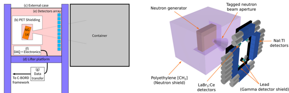
Fig. 1. General scheme of the C-BORD's tagged neutron inspection system (TNIS).
