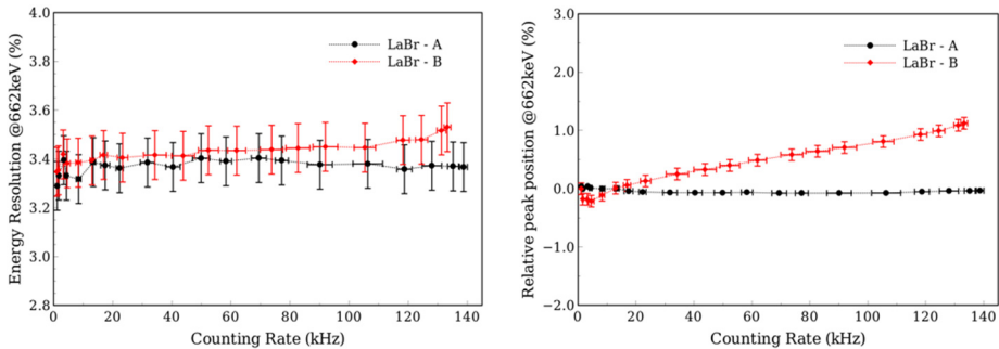
Fig. 6. (left) Energy resolution and (right) relative peak position at 662 keV as a function of the counting rate of the two 3 in \times 3 in LaBr 3 :Ce scintillators.
