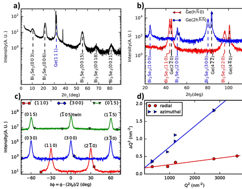
FIG. 3. (a) Out-of-plane symmetric \theta/2\theta spectrum close to the substrate reciprocal direction Ge(h\ h\ h) substrate. A small offset \delta\omega = \omega - \theta = 0.25^\circ was used to attenuate the substrate peaks and reduce the contribution from parasitic peaks ( K_\beta , \lambda/2 , ...) still present despite the K_\beta filtering. (b) In-plane GIXD radial scans along the two reciprocal directions separated from each other by 30^\circ : Ge(h\ \bar{h}\ 0) and Ge(2h\ \bar{h}\ \bar{h}) . The incidence angle was optimized to 0.32^\circ . (c) In-plane GIXD azimuthal scans for two peak families \{300\} and \{110\} . The spectra of \{100\} , \{200\} and \{220\} families were also measured but not shown here for clarity. The azimuthal scan of the \{015\} reflection shows the presence of twin domains. This measurement was performed using the same grazing incidence, 0.32^\circ , but with suitable exit angles. (d) Square of the FWHM of Bragg peaks (in Q units) as a function of the square of the momentum transfer Q for both in-plane radial and azimuthal scans. The two linear fits show equal intercepts at the origin giving an estimation of the domains size: D \approx 15 nm.
