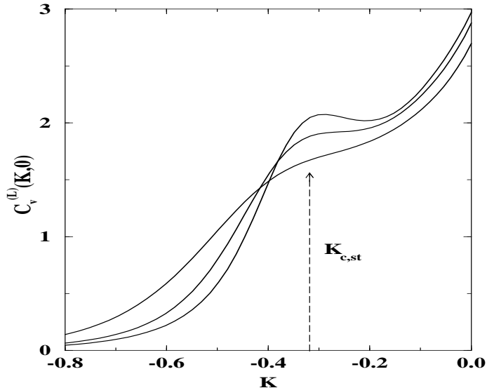
Fig. 11: Heat capacity C_v^{(L)}(K, 0) for L = 4, 6, 8 and K \in [-0.8, 0] .
