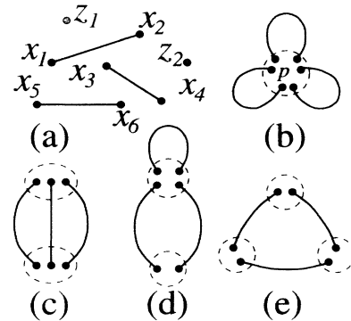
FIG. 1. A general diagram with two external points and three internal dipoles. (a) “Molecules” describing singular configurations with one (b), two (c) and (d), and three (e) “atoms.” (b)–(d) give uv divergences; (e) does not.
