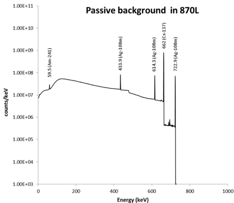
17 Fig. 10. Passive background spectrum of the 870L package (3 h counting).
