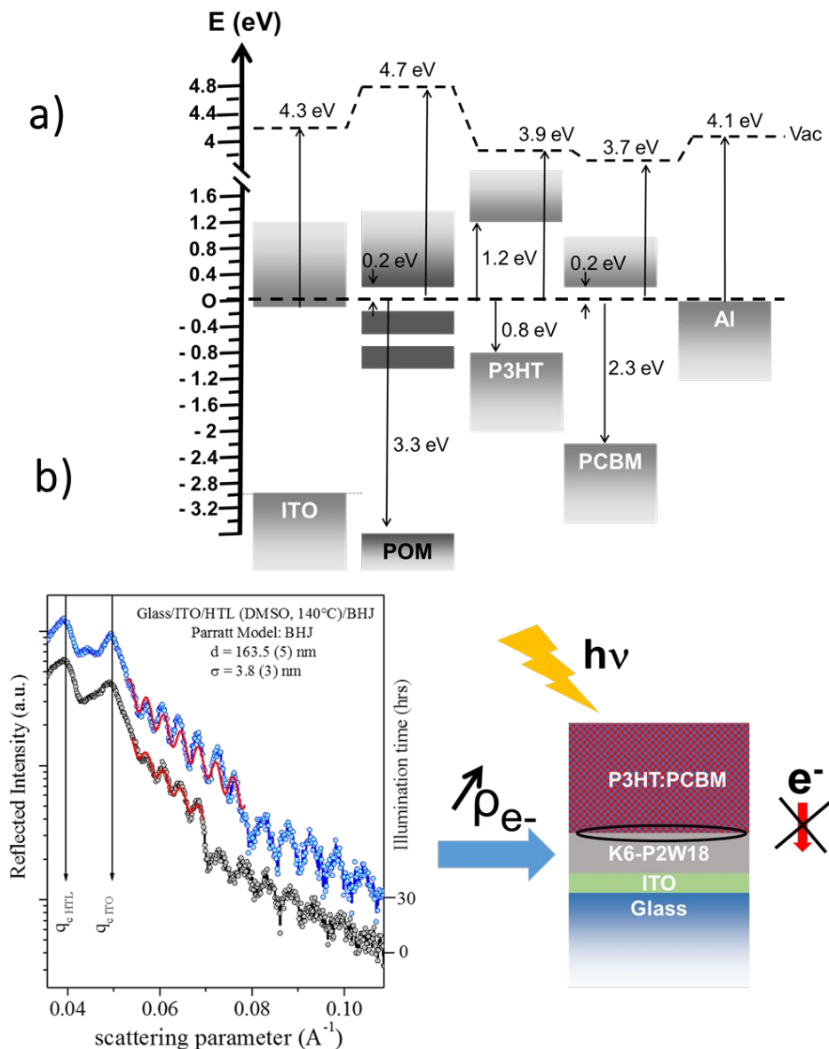
Figure 6. (a) Global energy band diagram of a P3HT:PCBM photovoltaic cell with the K6-P2W18 thin film at the ITO interface, and (b) EDXR patterns of glass/ITO/K6-P2W18/P3HT:PCBM and best fits, black curve correspond to dark measurement and blue curve to the measurement performed under illumination.
