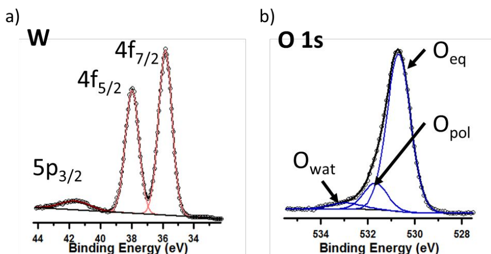
Figure 2. Photoelectron spectroscopy of an annealed 46 nm K6-P2W18 film grown on a glass/ITO substrate: XPS W 4f (a) and O 1s (b) core-level spectra.
