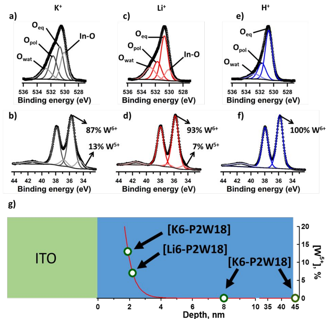
Figure 3. (a-f) O 1s and W 4f XPS spectra of 1.9 nm K6-P2W18 (a,b), 2.1 nm Li6-P2W18 (c,d) and 3.8 nm H6-P2W18 (e,f) films. (g) Variation of the percentage of W 5+ as a function of layer thickness.
