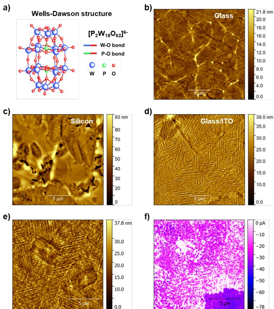
Figure 1. (a) Schematic representation of the Wells-Dawson type polyoxoanion [P_2W_{18}O_{62}]^{6-} . (b), (c) and (d) AFM topographic images of 46 nm K6-P2W18 films grown on glass (b), silicon (c) and glass/ITO (d) substrates. Topography (e) and current mapping (f) (bias = -600 mV) of a highly ordered K6-P2W18 film on glass/ITO.
