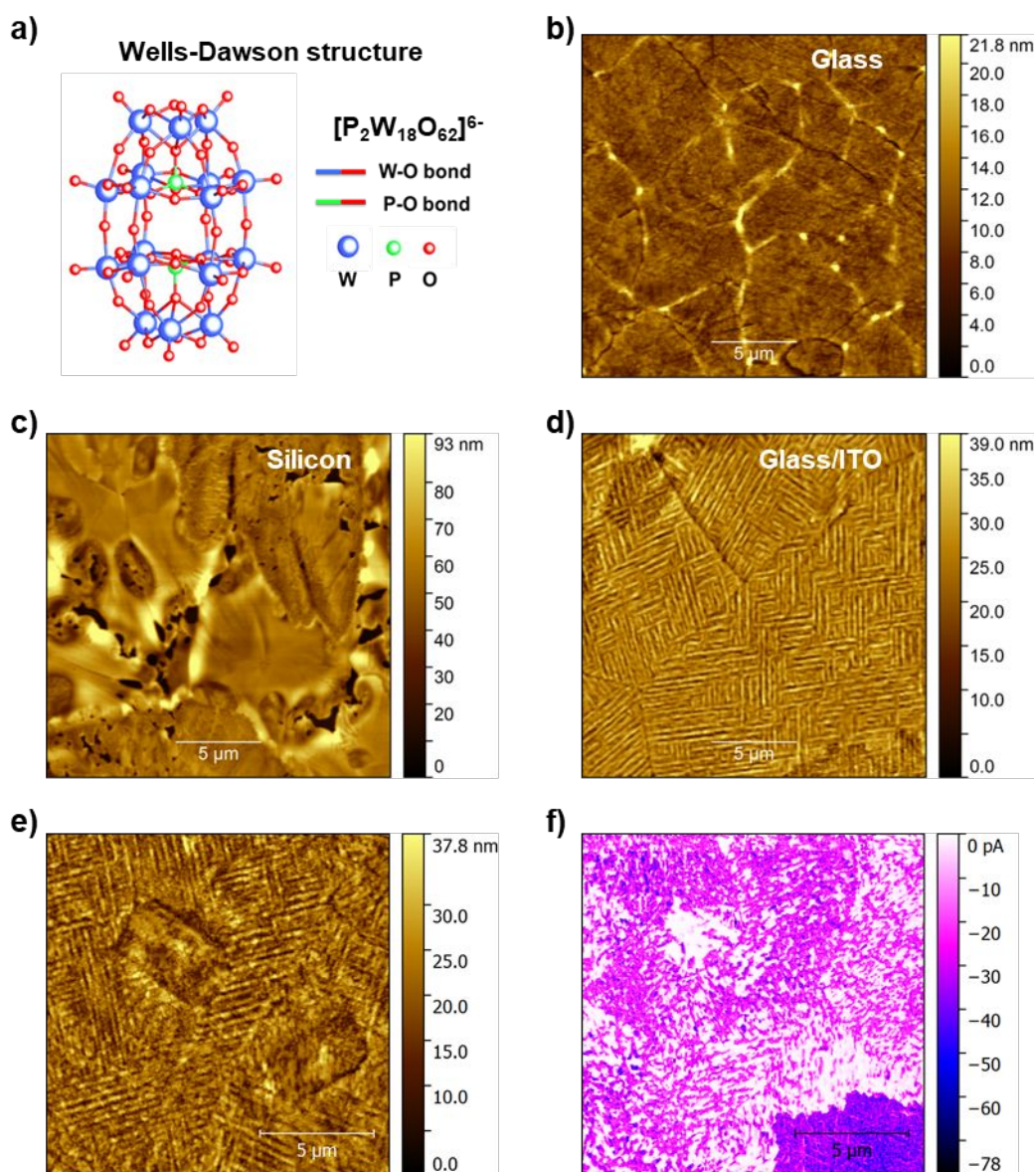
Figure 1. (a) Schematic representation of the Wells-Dawson type polyoxoanion [P 2 W 18 O 62 ] 6- . (b), (c) and (d) AFM topographic images of 46 nm K6-P2W18 films grown on glass (b), silicon (c) and glass/ITO (d) substrates. Topography (e) and current mapping (f) (bias = -600 mV) of a highly ordered K6-P2W18 film on glass/ITO.
