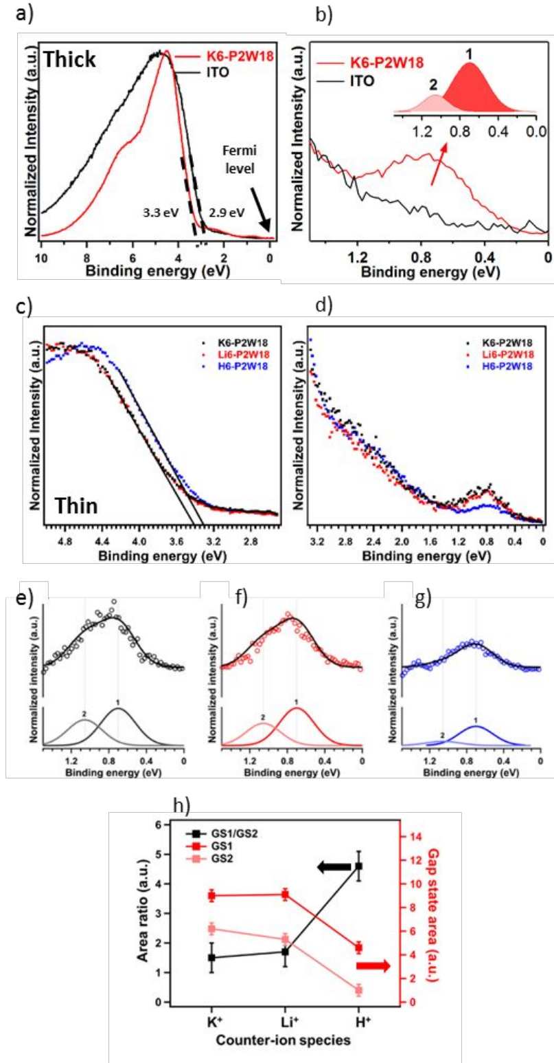
Figure 4. (a) Valence band spectra of a thick (> 46 nm) annealed K6-P2W18 film on ITO, (b) extraction and deconvolution of the gap state signal, (c) Spectra of thin K6-, Li6- and H6-P2W18 layers on ITO, (d) zoom on the energy region of the gap states, (e-f-g) deconvolution of the gap state signal into two components for each of the three thin layers, (h) intensity ratio of the two gap state components as a function of counter ion.
