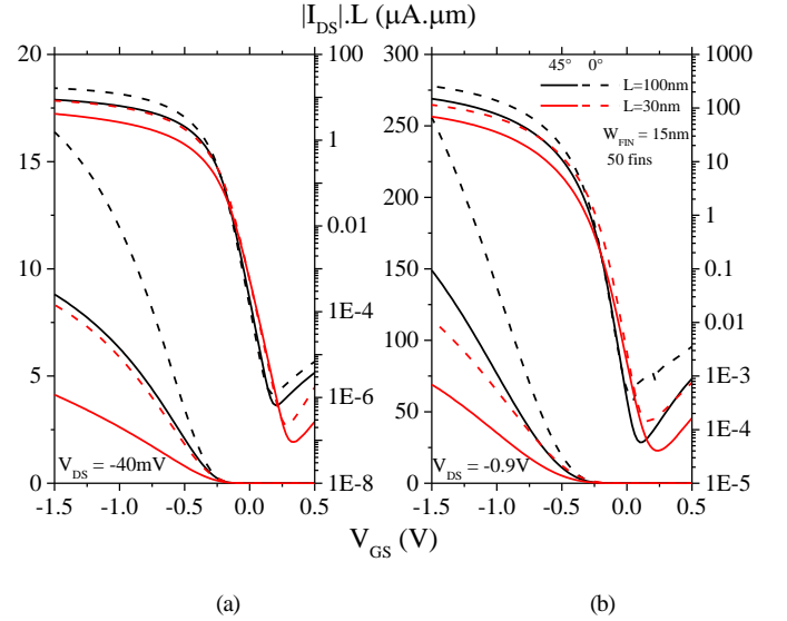
Fig.3. |I_{DS}|L as a function of V_{GS} at V_{DS} = -40\text{mV} (a) and -0.9\text{V} (b) for [110] and [100]-NWs, L = 100 and 30\text{nm} .
