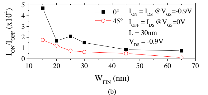
Fig.4. I_{ON}/I_{OFF} characteristics for [110] and [100]-NWs with L = 30\text{nm} , at V_{DS} = -0.9\text{V} .
