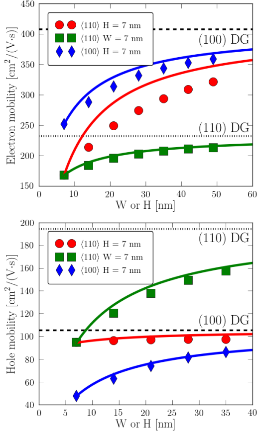
Fig. 1. Electron (upper panel) and hole (lower panel) mobilities in rectangular (100) and (110) GAA SiNWs as a function of width ( W ) or height ( H ) at carrier density n = 8 \times 10^{12} \text{ cm}^{-2} . The symbols are the NEGF results. The dashed and dotted horizontal lines are the NEGF reference mobilities in (100) and (110) DG devices, respectively. The solid lines are the interpolations from SQGAA NW devices to the limiting DG devices using Eq. (2).
