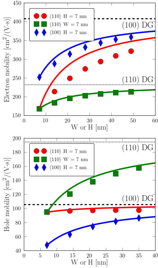
Fig. 1. Electron (upper panel) and hole (lower panel) mobilities in rectangular (100) and (110) GAA SiNWs as a function of width ( W ) or height ( H ) at carrier density n = 8 \times 10^{12} \text{ cm}^{-2} . The symbols are the NEGF results. The dashed and dotted horizontal lines are the NEGF reference mobilities in (100) and (110) DG devices, respectively. The solid lines are the interpolations from SQGAA NW devices to the limiting DG devices using Eq. (2).
