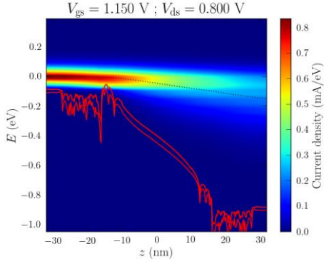
Fig 8: Spectral density of current along the nanowire axis at V_{ds} = 0.8 V and in strong inversion for a W = 10 \times H = 10 nm Trigate device with 20 nm gate length. The red lines are the conduction band profiles of the X, Y and Z valleys.
