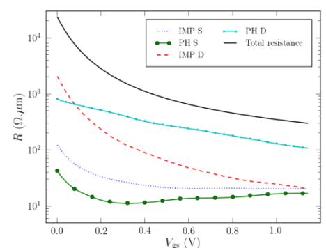
Fig 9: Contributions of scattering by phonons (PH) and by impurities (IMP) in the source (S) and drain (D) to the total resistance at V_{ds} = 0.8 V in a W = 10 \times H = 10 nm Trigate device with 20 nm gate length. The total resistance includes the channel resistance.
