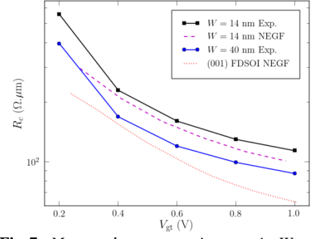
Fig 7: Measured contact resistances in W = 40 \times H = 12 nm and W = 14 \times H = 12 nm Trigate devices, as a function of gate overdrive. They are compared with simulations for a planar (001), 12 nm thick FDSOI device and for a W = 14 \times H = 12 nm Trigate device.
