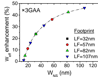
Fig. 8: W_{eff} enhancement (compared to FF with FP=25 \text{ nm} ) vs. W_{NS} for different layout footprints (LF). Here, H_{NS}=H_{NW}=6.3 \text{ nm} (cf. Fig. 3).
