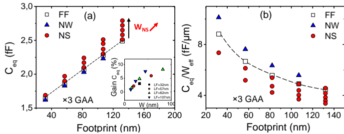
Fig.14: (a) Effective load capacitance C_{eq} as a function of LF for FF (with FP=25\text{nm} ) and stacked-NW/NS structures. The larger the footprint is, the wider the NS will be, resulting in larger C_{inv} contribution at high W_{eff} . However, the normalized effective load capacitance is significantly reduced for NS (b).
