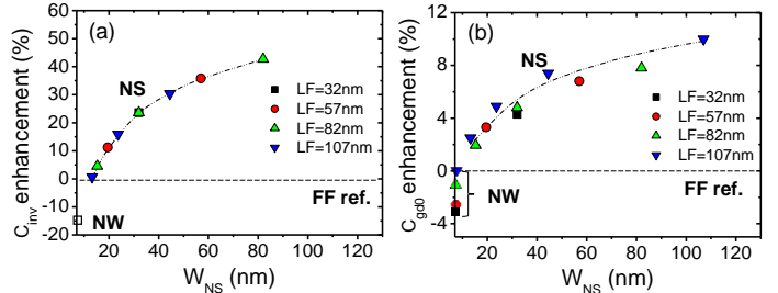
Fig.13: C_{inv} (a) and C_{gdo} (b) enhancement over FinFET (with FP=25\text{nm} ) for stacked-NS/NW structures. Capacitances are calculated for different layout footprints (LF). Whatever the LF, C_{inv} and C_{gdo} increase with W_{NS} (+28% improvement for C_{inv} against only +6% for C_{gdo} at W_{NS}=40\text{nm} ).
