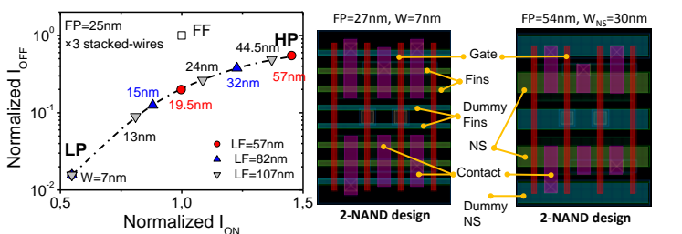
Fig.19: Normalized I_{OFF} vs. I_{ON} current (over FinFET with FP=25\text{nm} ) for L_G=16\text{nm} . A tuning of the NS width allows one to modulate the threshold voltage and the subthreshold slope, enabling a better performance-power optimization.
