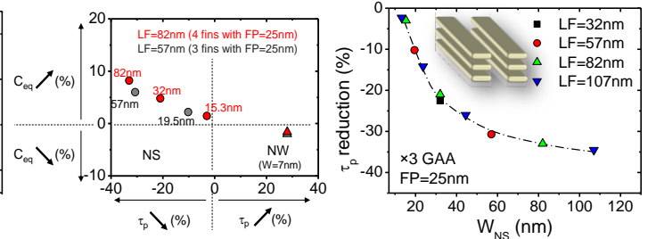
Fig.15: \tau_p and C_{eq} reduction over FinFET (with FP=25\text{nm} ) technology for different LF. A \tau_p reduction of ~20% is expected at W_{NS}=30\text{nm} .
