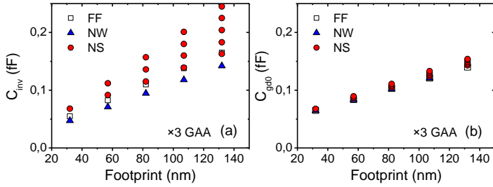
Fig.12: Inversion (a) and gate-to-drain (b) capacitances vs. layout footprint for FF and stacked-NW/NS structures. As compared to FF (with FP=25\text{nm} ) devices, an increase of W_{NS} for a constant footprint results in a C_{inv} enhancement due to higher W_{eff} . However, a small improvement of C_{gdo} is observed as W_{NS} increases.
