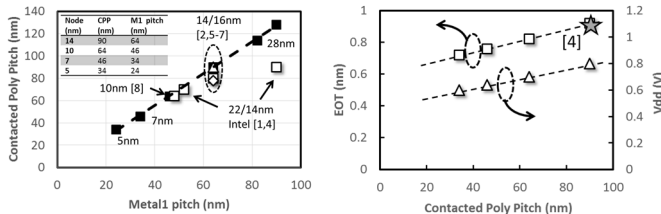
Fig. 7: Fig. 1. Contacted poly pitch versus metal1 pitch (Left) and Equivalent Oxide Thickness vs supply voltage (Right)
