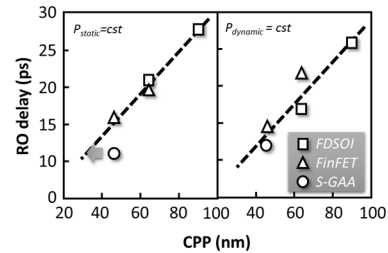
Fig. 9. RO delay versus nodes CPP for all architectures. Symbols are RO simulations, dashed line is the trend of +35% on speed per node.
