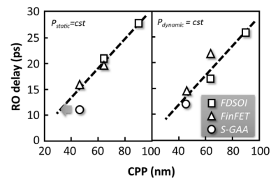
Fig. 9. RO delay versus nodes CPP for all architectures. Symbols are RO simulations, dashed line is the trend of +35% on speed per node.
