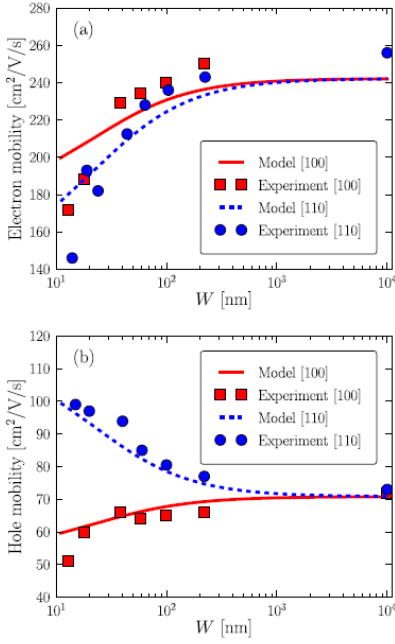
Fig. 3: Electron (a) hole (b) long channel mobility models as a function of device's width in rectangular Trigate devices ( H = 11 nm), at carrier density n = 10^{13} \text{cm}^{-2} . The symbols are the experimental data, while the solid and dashed lines are the interpolated long channel mobility models
