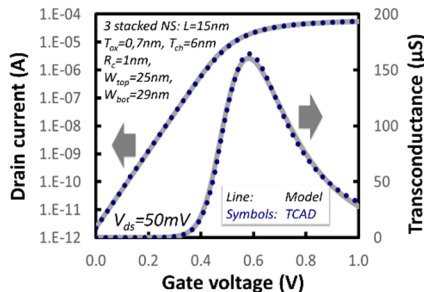
Fig. 15. Drain current and its derivative vs gate voltage of SNS GAA MOSFET in linear regime for the validation of model's core.
