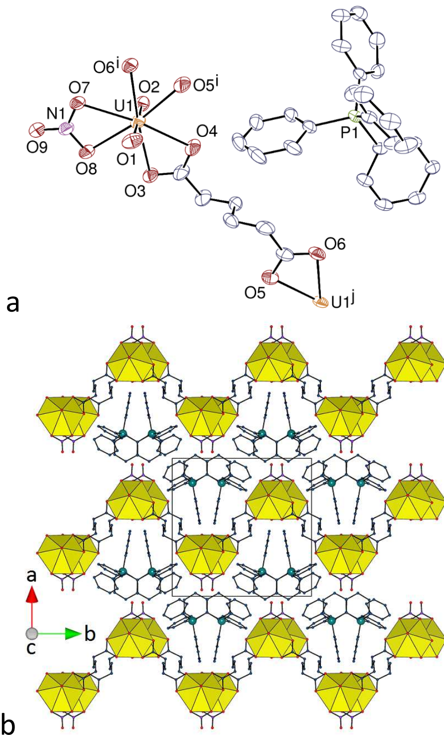
Figure 1. (a) View of compound 1 . Displacement ellipsoids are drawn at the 50% probability level. Symmetry codes: i = 1 - x, y + 1/2, 3/2 - z ; j = 1 - x, y - 1/2, 3/2 - z . (b) View of the packing with uranium coordination polyhedra colored yellow. Hydrogen atoms are omitted in both views.
