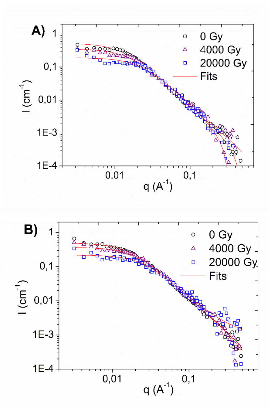
Figure 3. SANS spectra of (A) PMAA-AuNPs and (B) P(HEMA-MAA)-AuNPs, before and after irradiation.
