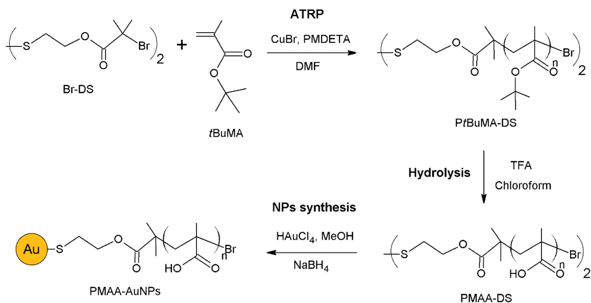
Scheme 1. Synthesis of PMAA-grafted gold nanoparticles (PMAA-AuNPs).
