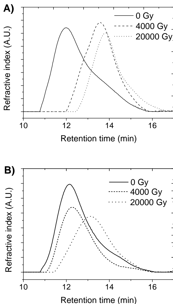
Figure 4. Irradiation effects on PMAA-AuNPs: SEC measurements after irradiation of degrafted polymer chains from (A) PMAA-AuNPs and (B) P(HEMA-MAA)-AuNPs.
