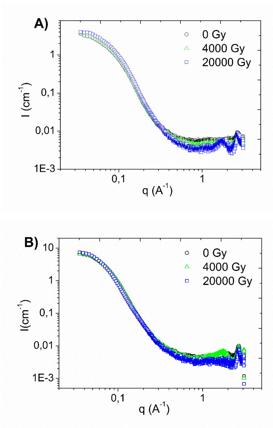
Figure 2. SAXS spectra of polymer-grafted AuNPs (10 mg/mL solutions in water) before and after irradiation: (A) PMAA-AuNPs and (B) P(HEMA-MAA)-AuNPs.
