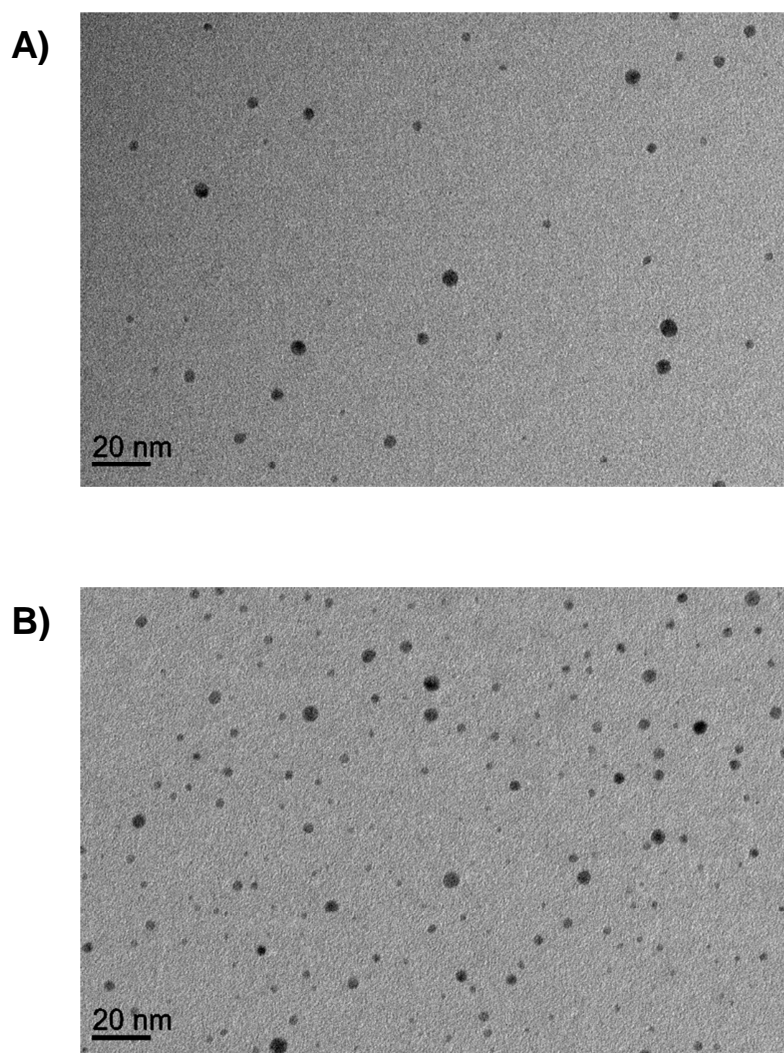
Figure 1. TEM micrograph of (A) PMAA-AuNPs and (B) P(HEMA-MAA)-AuNPs.
